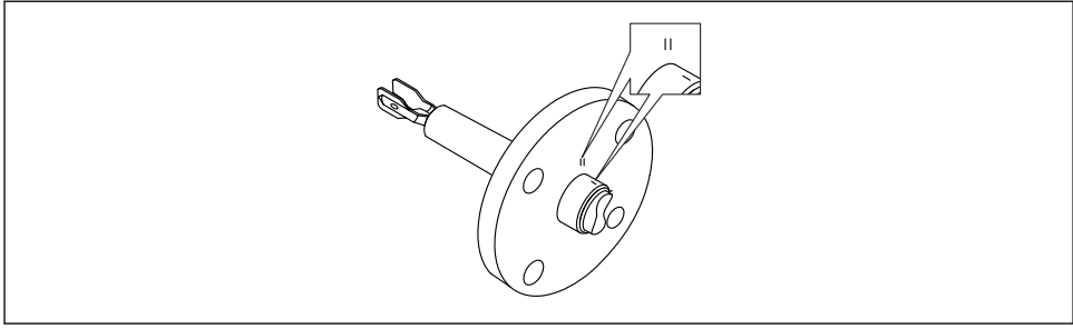
11 Position of the tuning fork when installed horizontally in the vessel using the marking
