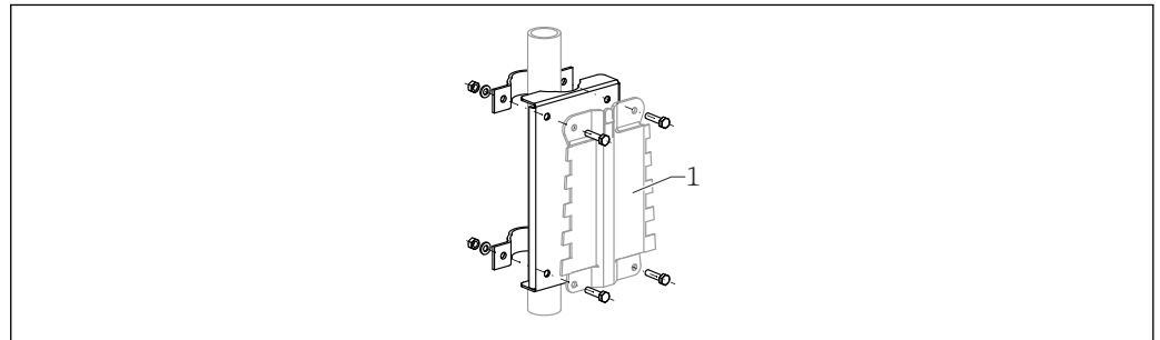
13 Mounting plate for polycarbonate field housing
