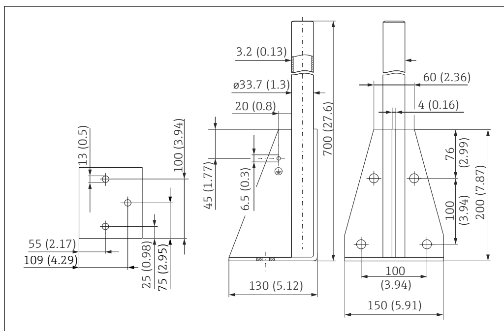
14 Dimensions. Unit of measurement mm (in)
