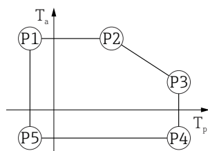
图 35 铝外壳, 带涂层; 过程温度范围: -10 \dots +200 \text{ }^{\circ}\text{C} ( +14 \dots +392 \text{ }^{\circ}\text{F} )
