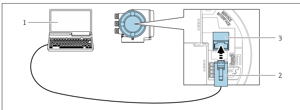
55 Raccordement via interface service (CDI-RJ45)
