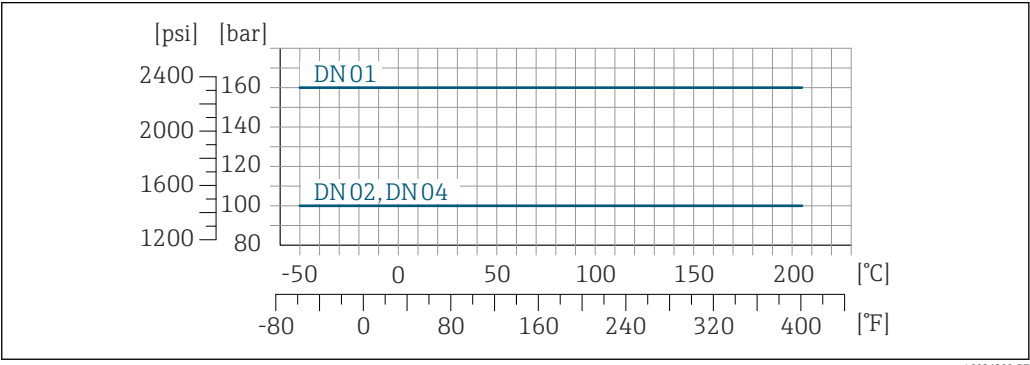
29 Com material do flange: 1.4404 (316/316L)
