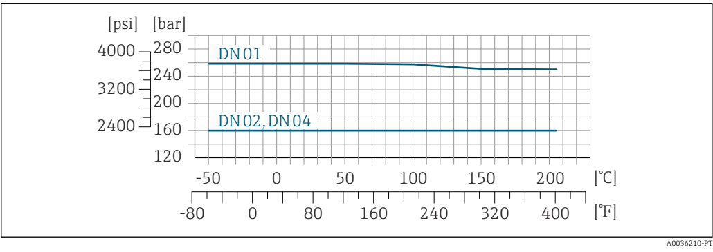
30 Com material do flange: Liga C22, 2.4602 (UNS N06022)
