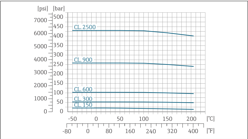
25 Com material do flange: Liga C22, 2.4602 (UNS N06022)
