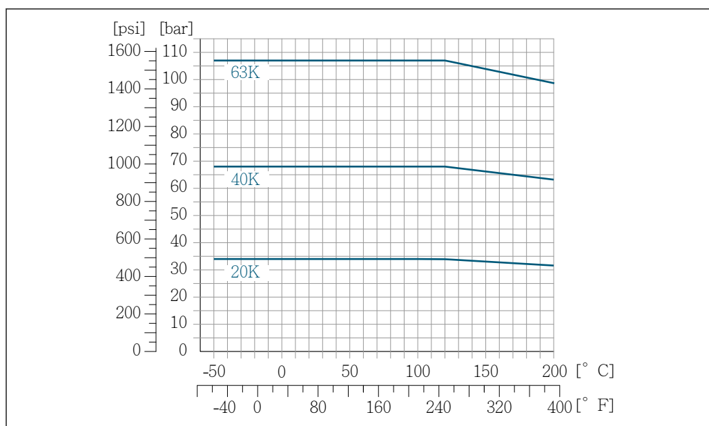
27 Com material do flange: 1.4404 (316/316L) ou Liga C22, 2.4602 (UNS N06022)
