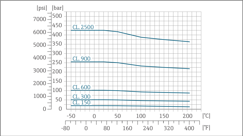
24 Com material do flange: 1.4404 (316/316L)
