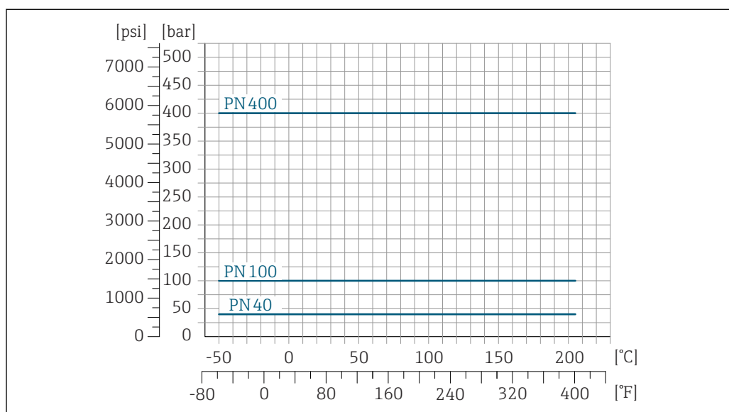
22 Com material do flange: Liga C22, 2.4602 (UNS N06022)
