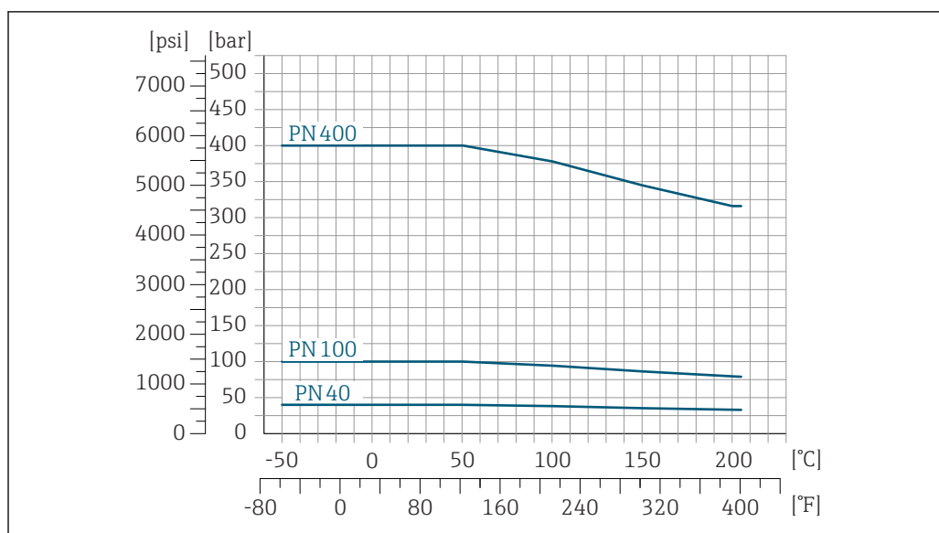
21 Com material do flange: 1.4404 (316/316L)
