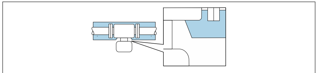
31 Thermal insulation with exposed extension neck
