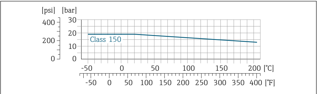
23 With flange material 1.4404 (F316/F316L)
