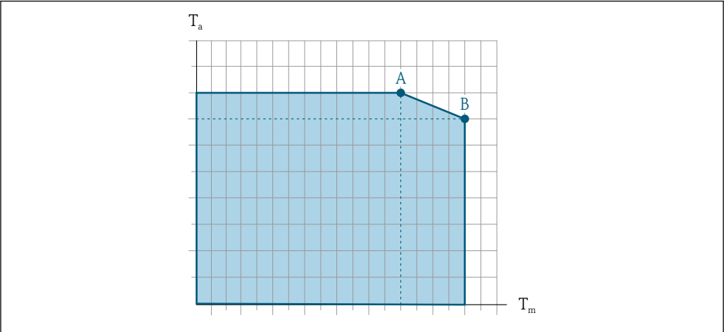
21 Exemplary representation, values in the table below. T_a Ambient temperature T_m Medium temperature A Maximum permitted medium temperature T_m at T_{a\ max} = 60\ ^\circ\text{C} (140 °F); higher medium temperatures T_m require a reduction in the ambient temperature T_a B Maximum permitted ambient temperature T_a for the maximum specified medium temperature T_m of the sensor
