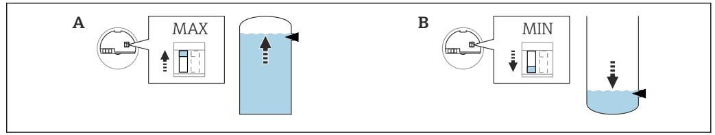
45 Switch position on the electronic insert for MAX/MIN safety mode
