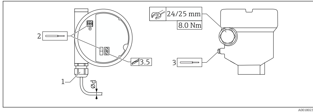
32 Example of coupling with cable entry, electronic insert with terminals
