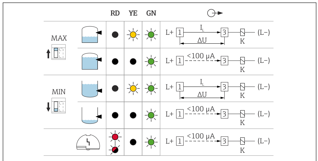
21 Behavior of switch output and signaling, electronic insert FEL62
