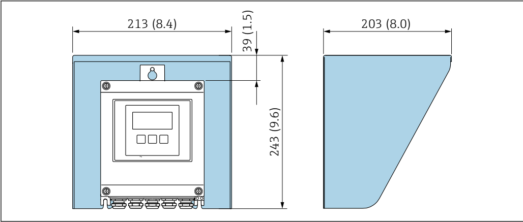
19 Protective cover for Proline 500 – digital; unit mm (in)
