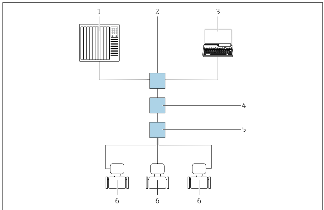
32 Options for remote operation via Modbus TCP over Ethernet-APL protocol (active)
