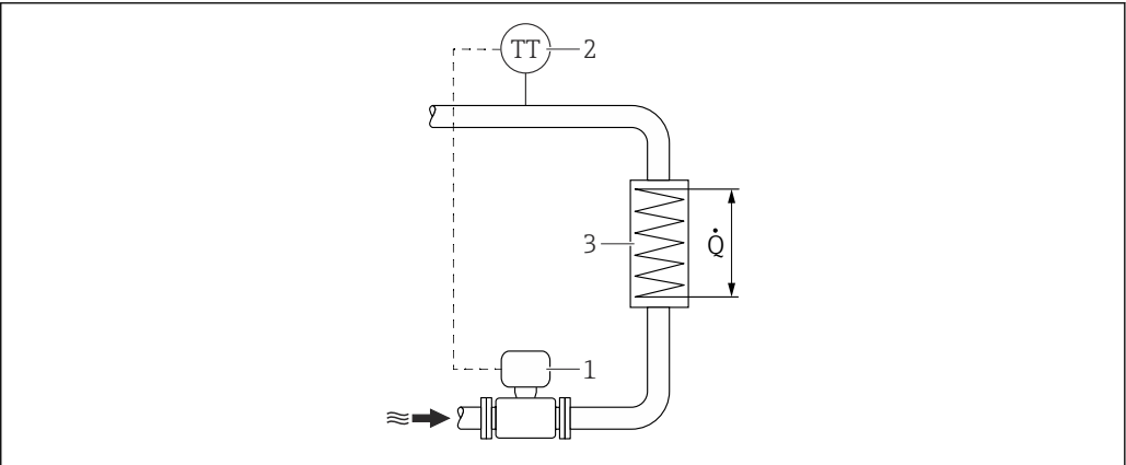
15 Layout for delta heat measurement of saturated steam and water 1 Measuring instrument 2 Temperature sensor 3 Heat exchanger Q Heat flow
