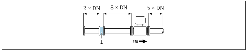
1 Flow conditioner
