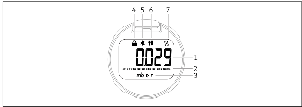
6 Segment display
