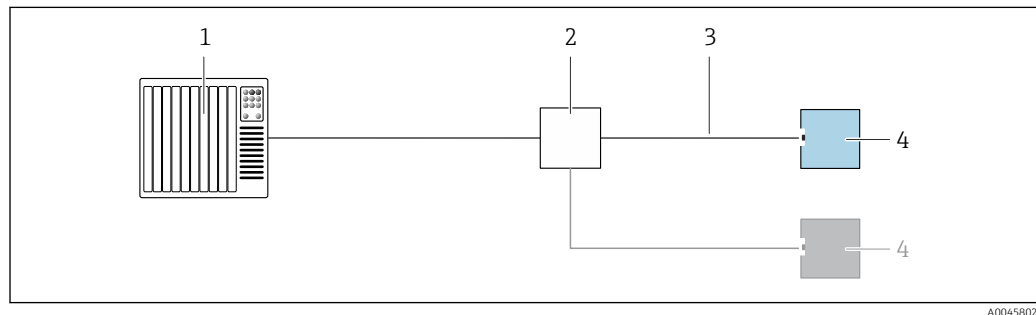
4 Connection example for PROFINET over Ethernet-APL
