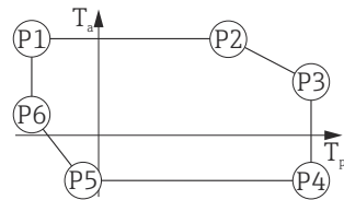
▣ 37 铝外壳, 带涂层; 过程温度: -196 \dots +200 \text{ }^{\circ}\text{C} ( -320 \dots +392 \text{ }^{\circ}\text{F} )
