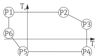
图 28 塑料外壳; 过程温度: -196 \dots +200 \text{ }^{\circ}\text{C} ( -320 \dots +392 \text{ }^{\circ}\text{F} )
