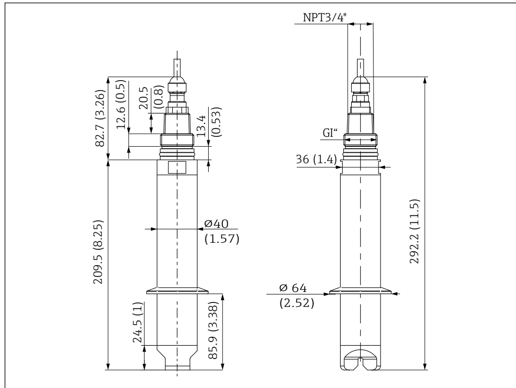
16 Dimensions with clamp. Dimensions: mm (in)
