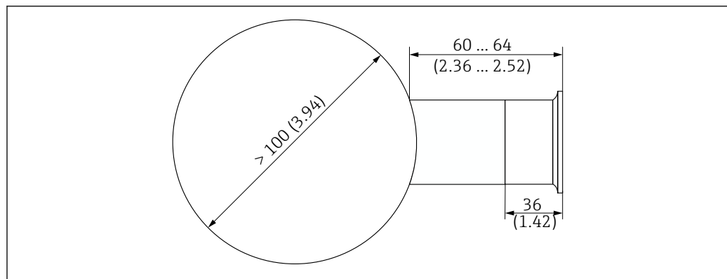
19 Pipe connection with weld-in adapter. Unit: mm (in)
