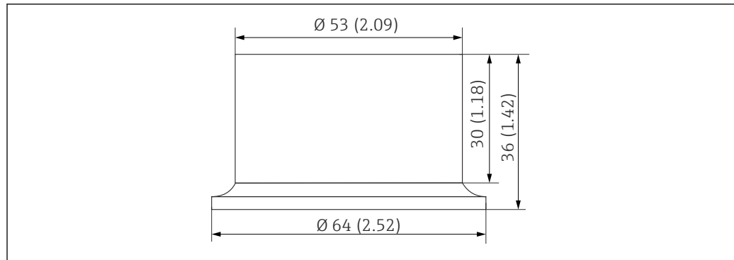
18 Weld-in adapter. Unit: mm (in)
