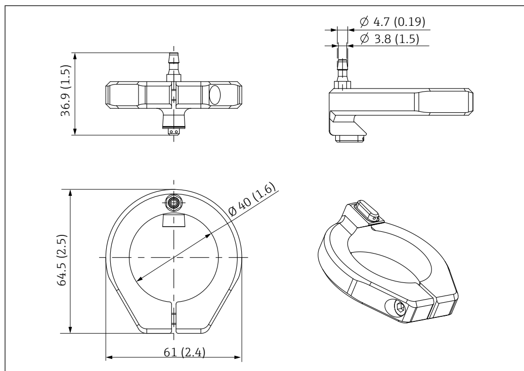
17 Dimensions for compressed air cleaning. Dimensions: mm (in)
