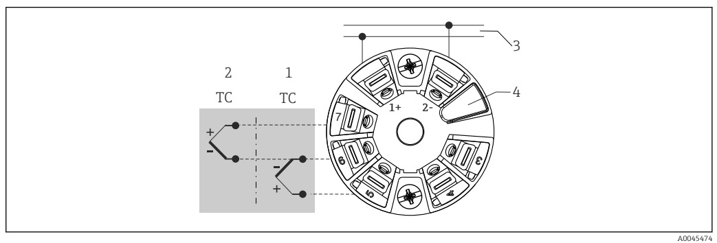
8 Head-mounted transmitter TMT8x (dual sensor input)
