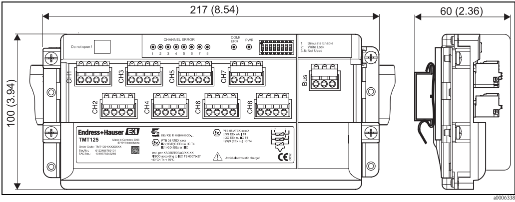
Housing for DIN rail as per IEC 60715; specifications in mm (inch)
