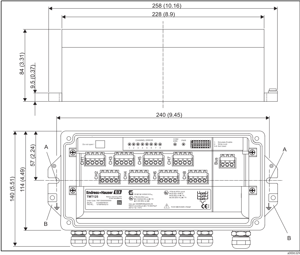
Dimensions of field housing; specifications in mm (inch)
