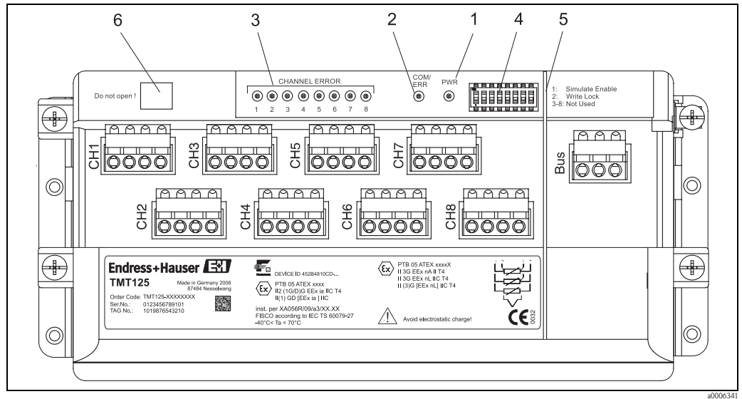
Operating and display elements of the temperature transmitter
