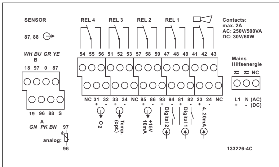
11 Autocollant du compartiment de raccordement Liquisys M, version WX/WS
