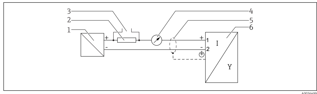
10 Blockdiagramm 2-Draht: 4-20 mA HART
