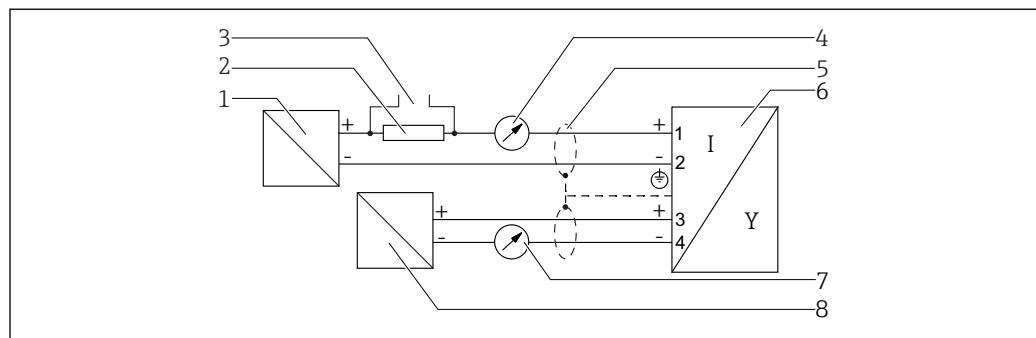
14 Blockdiagramm 2-Draht: 4-20 mA HART, 4-20 mA
