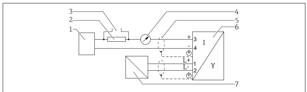
16 Blockdiagramm 4-Draht: 4-20 mA HART (10,4 ... 48 V DC )
