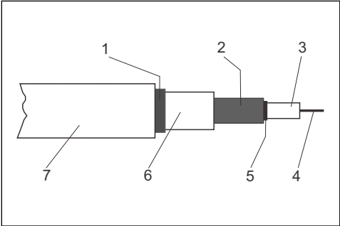
13 Structure of cable CYK71
