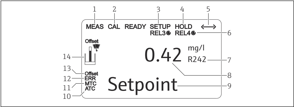
15 Transmitter LC display
