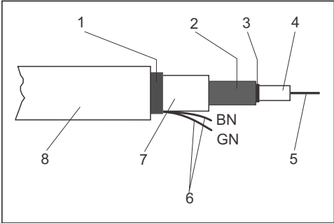
12 Structure of cable CMK
