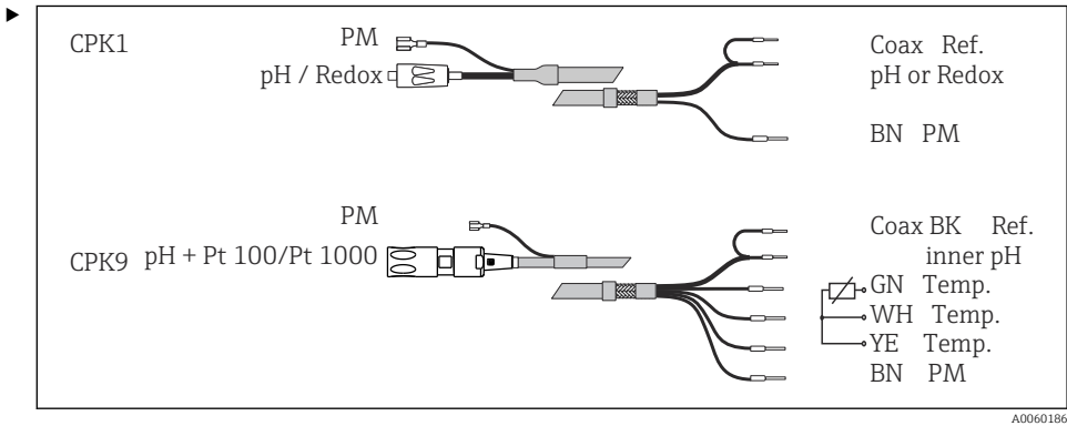
11 Connecting a pH/ORP sensor with CPK1 or CPK9 cables
