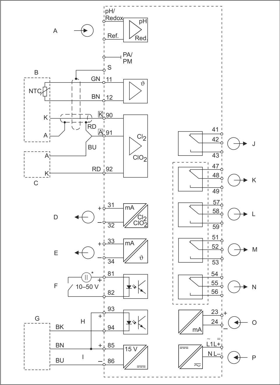
7 Electrical connection of the transmitter (version 1)
