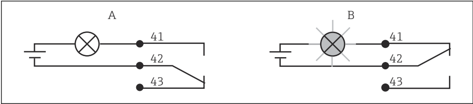
14 Recommended fail-safe switching for the alarm contact
