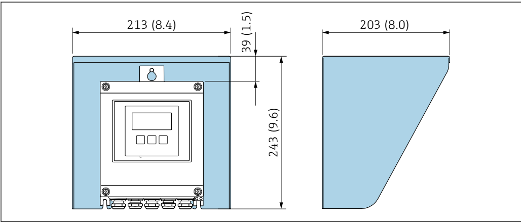
34 Weather protection cover for Proline 500 – digital; unit mm (in)
