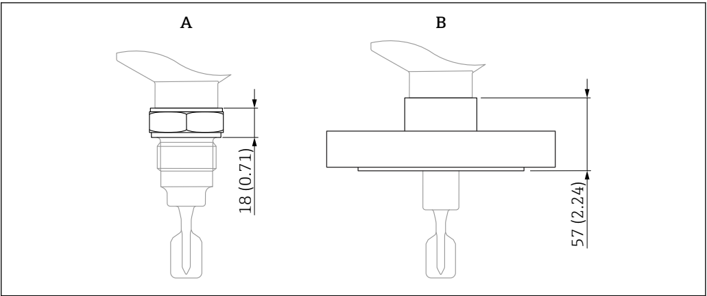
41 Maximum height specification for the process connections
