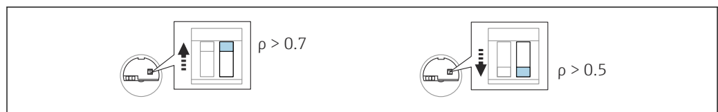
51 Switch position on the electronic insert for density
