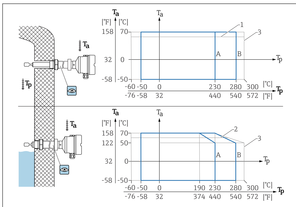
29 Permitted ambient temperature T_a at the housing as a function of the process temperature T_p in the vessel
