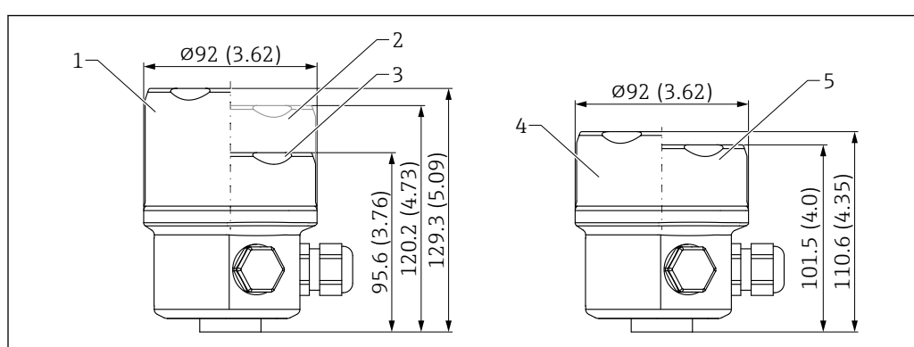
35 Dimensions of single-compartment housing, 316L, hygienic. Unit of measurement mm (in)
