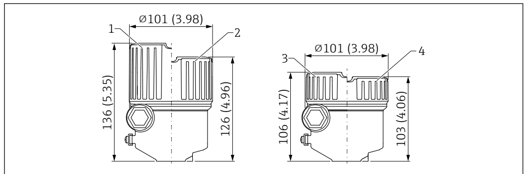
32 Dimensions of single-compartment housing, aluminum, coated. Unit of measurement mm (in)
