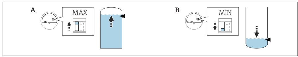
50 Switch position on the electronic insert for MAX/MIN safety mode
