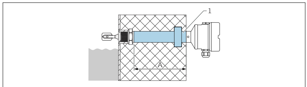
37 Temperature spacer with gas-tight glass feedthrough
