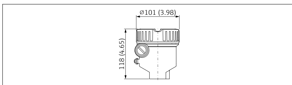
34 Dimensions of single compartment 316L housing; with Ex d/XP also, dust ignition-proof; cover without sight glass. Unit of measurement mm (in)
