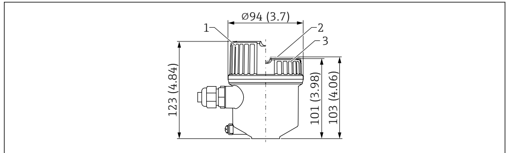
31 Dimensions of single compartment housing, plastic. Unit of measurement mm (in)
