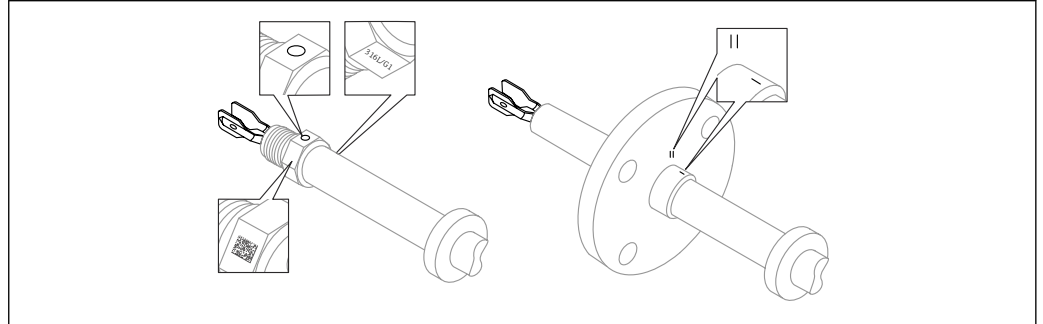
23 Position of the vibrating fork when installed horizontally in the vessel using the marking
