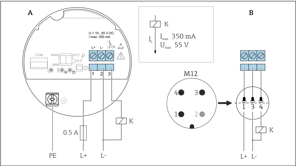
5 3-wire DC-PNP, electronic insert FEL62 A Connection wiring with terminals B Connection wiring with M12 plug in housing according to EN61131-2 standard
