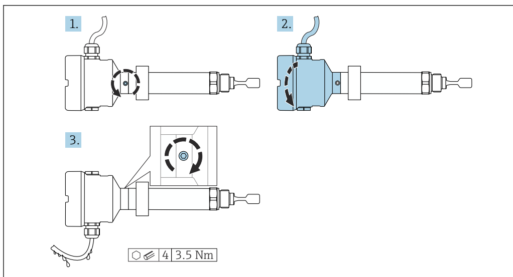
26 Housing with external locking screw and drip loop
