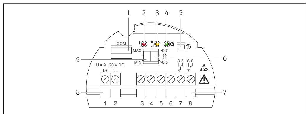
49 Example of electronic insert FEL64DC
