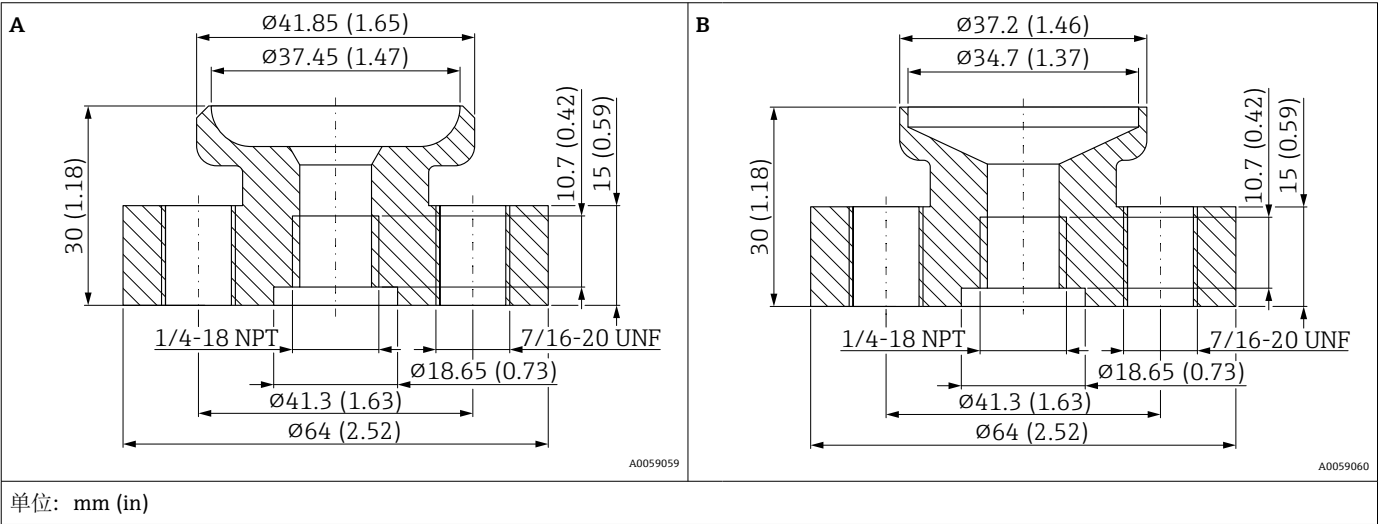
NPT1/4-18, 竖直安装, UNF7/16-20
