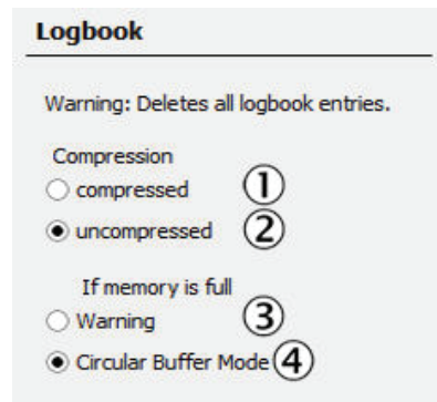
Figure 86: Menu Logbook
