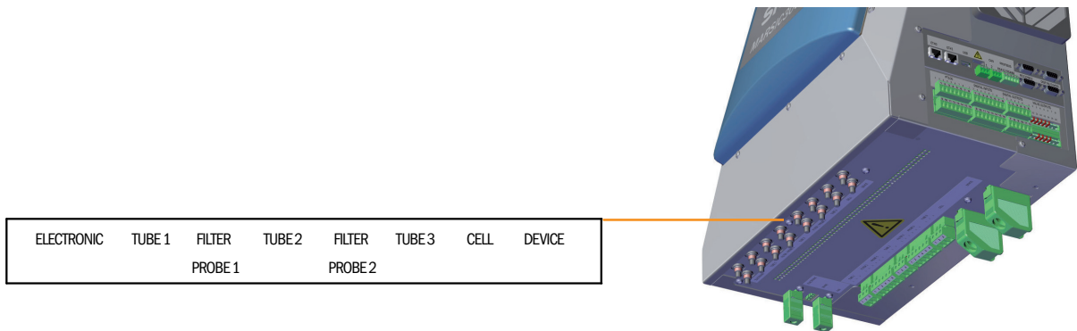
Figure 125: Electronics connections
