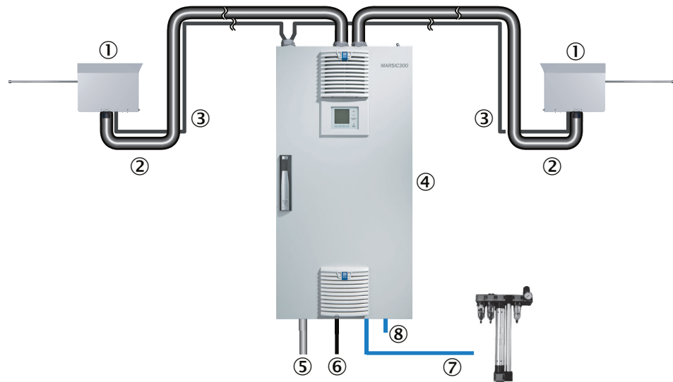
Figure 4: Installation - overview
