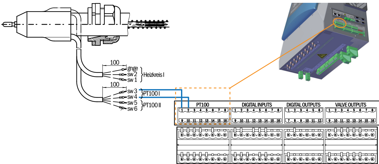
Figure 10: Pt100 connection
