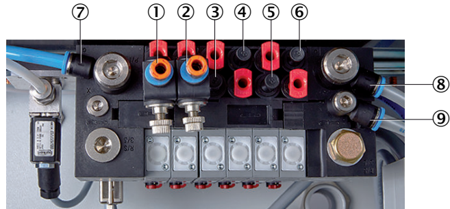
Figure 13: Valve block
