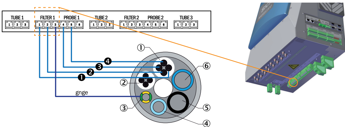
Figure 14: Supply lines - tube bundle cable connection diagram
