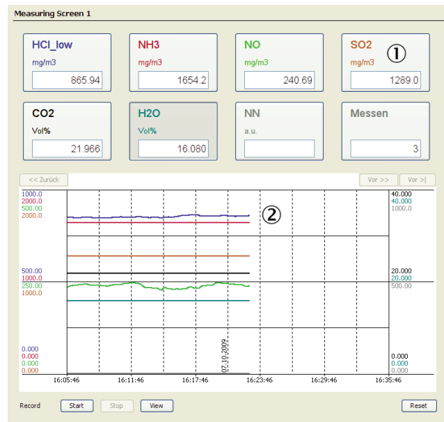
Figure 51: Line Writer
