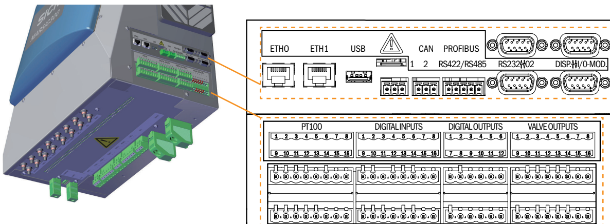
Figure 22: Connections overview
