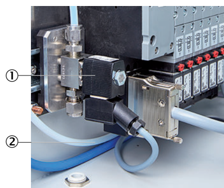
Figure 19: Test gas valve connection
