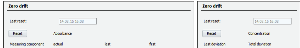
Figure 89: Menu Zero drift
