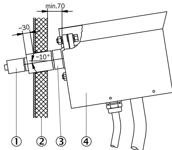
Figure 23: Flange assembly
