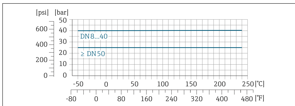
26 With connection material 1.4404 (316/316L)
