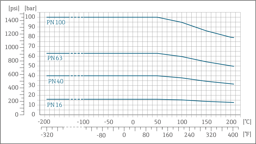
22 With flange material 1.4404 (F316/F316L)
