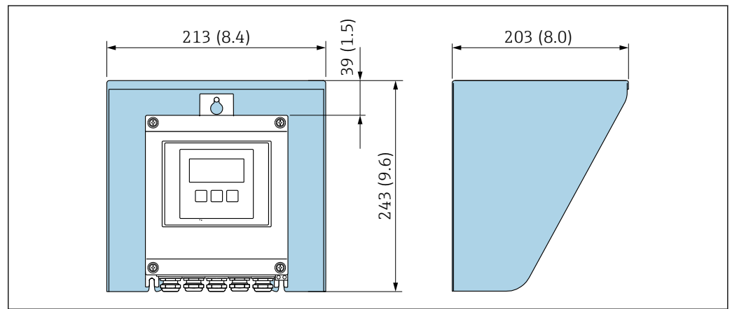
39 Weather protection cover for Proline 500 – digital; unit mm (in)
