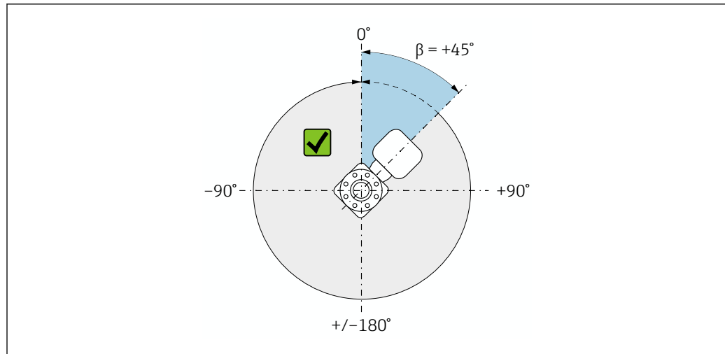
20 Top view in flow direction
