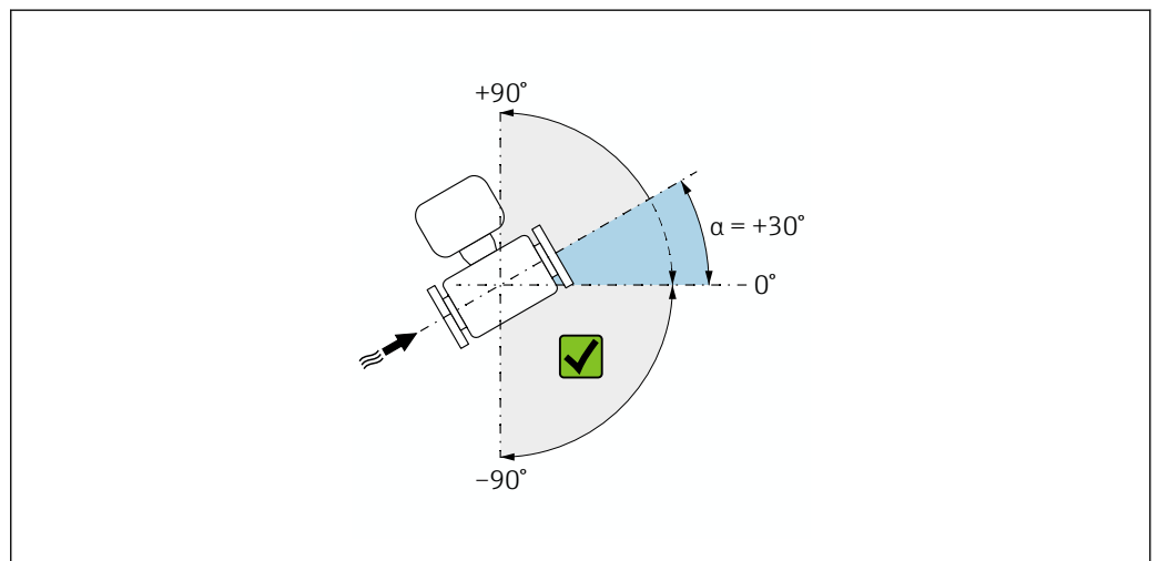
19 Side view with flow direction from left to right.
