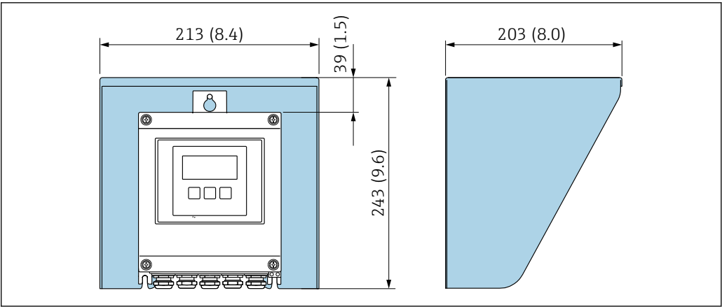
32 Weather protection cover for Proline 500 – digital; unit mm (in)
