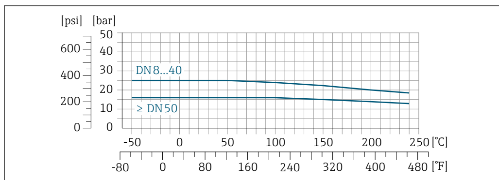
25 With connection material 1.4404 (316/316L)
