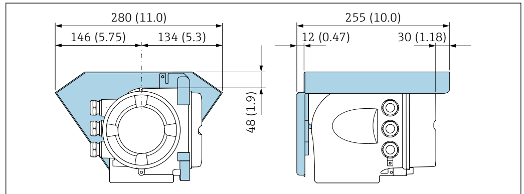
40 Weather protection cover for Proline 500 – unit mm (in)
