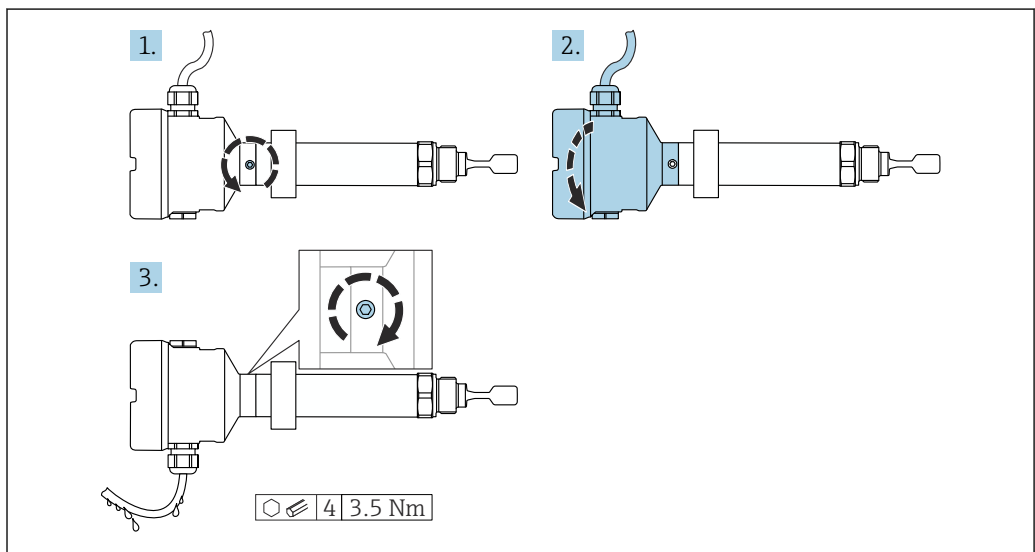
17 Housing with external locking screw and drip loop
