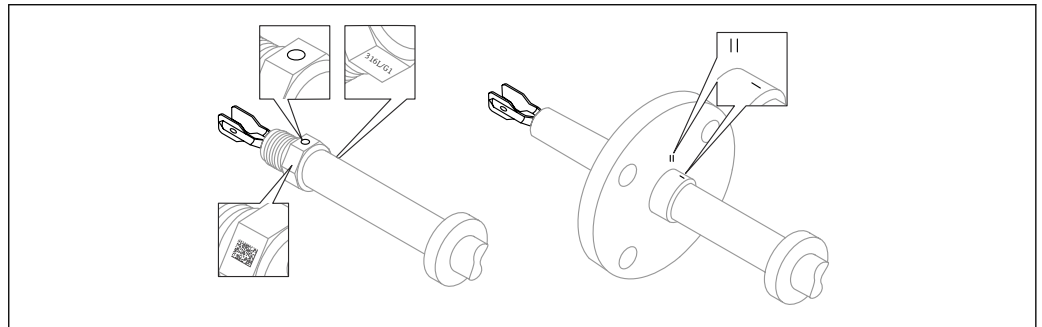
14 Position of the vibrating fork when installed horizontally in the vessel using the marking
