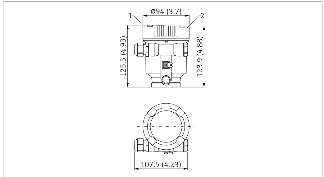
22 Dimensions; single compartment housing, plastic; incl. M20 coupling and plug, plastic. Unit of measurement mm (in)
