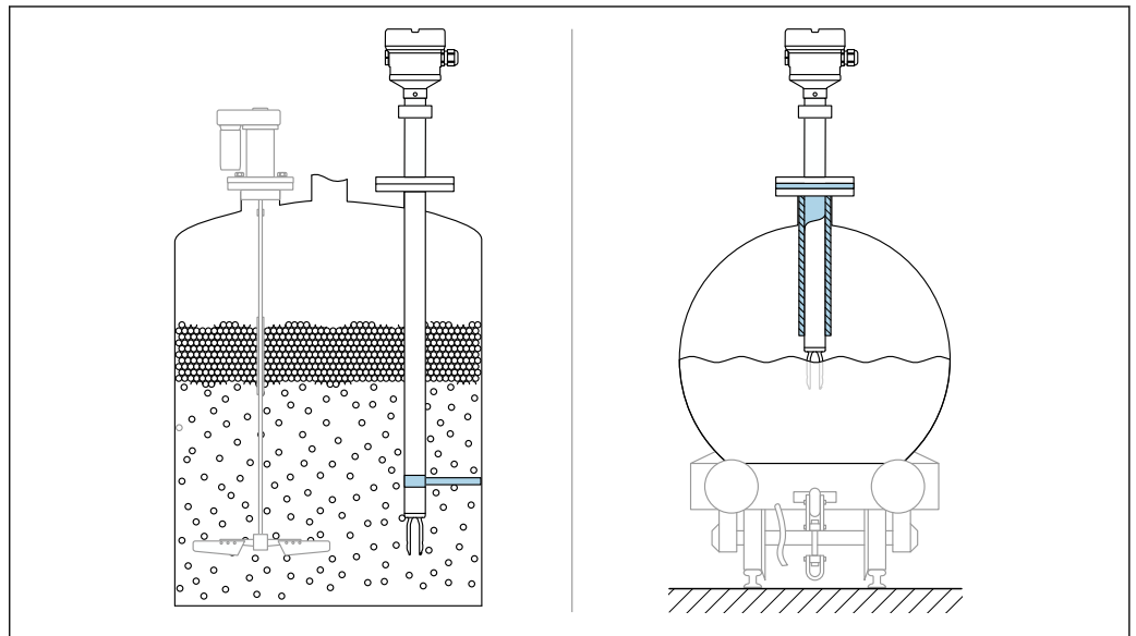
19 Examples of support in the event of dynamic load
