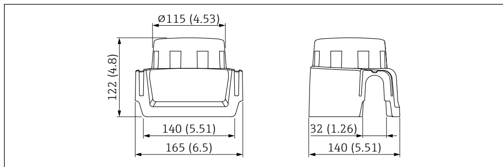
45 Dimensions of weather protection cover, plastic, XW111. Unit of measurement mm (in)
