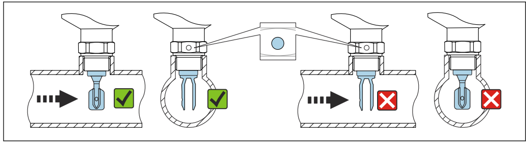
15 Installation in pipes (take fork position and marking into consideration)
