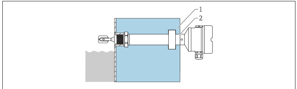
18 Vessel with heat insulation
