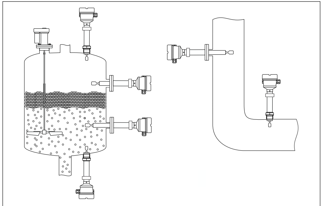
9 Installation examples for a vessel, tank or pipe
