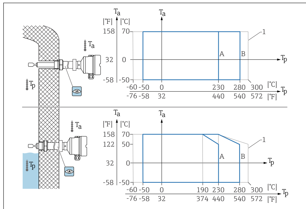
📘 20 Permitted ambient temperature T_a at the housing as a function of the process temperature T_p in the vessel
