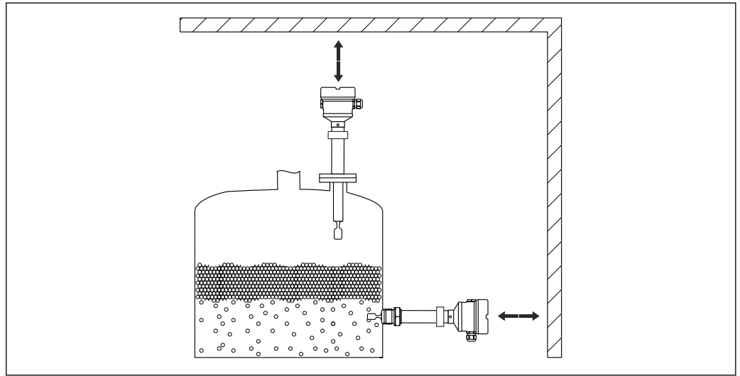
13 Take clearance into consideration
