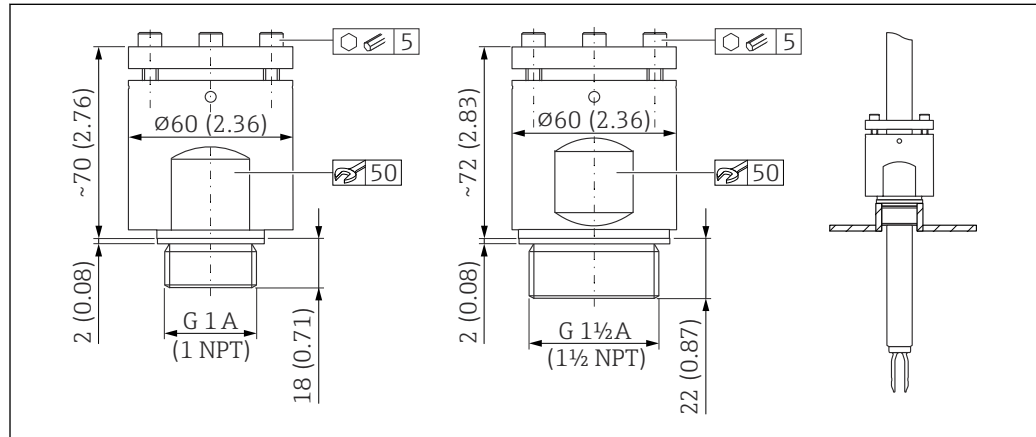
47 High pressure sliding sleeves. Unit of measurement mm (in)
