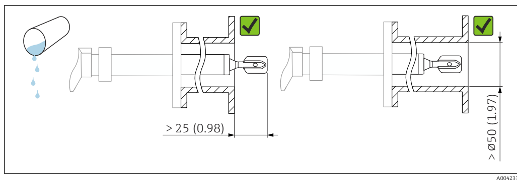
10 Installation example for low-viscosity liquids. Unit of measurement mm (in)
