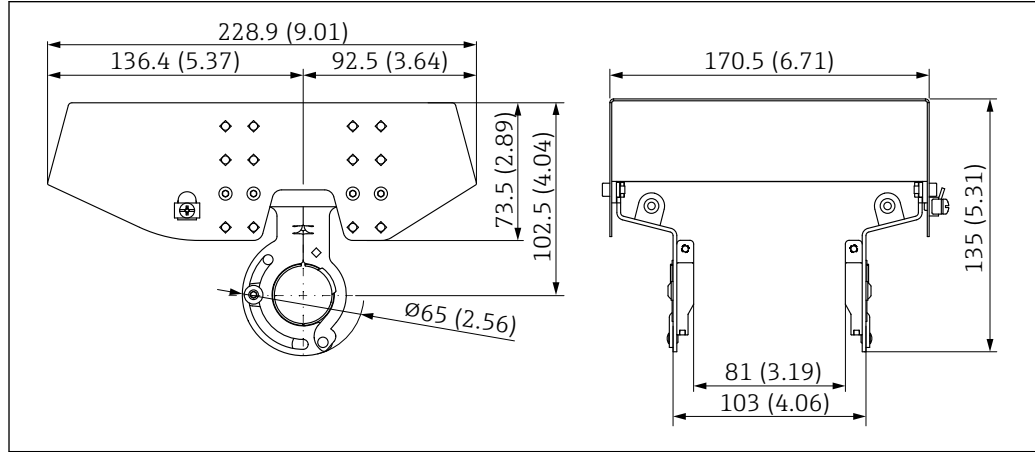
44 Dimensions of weather protection cover, 316 L, XW112. Unit of measurement mm (in)
