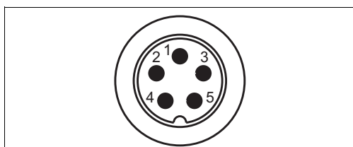
Fig. 73: Multihose connector M2 (Pg 21) at housing
