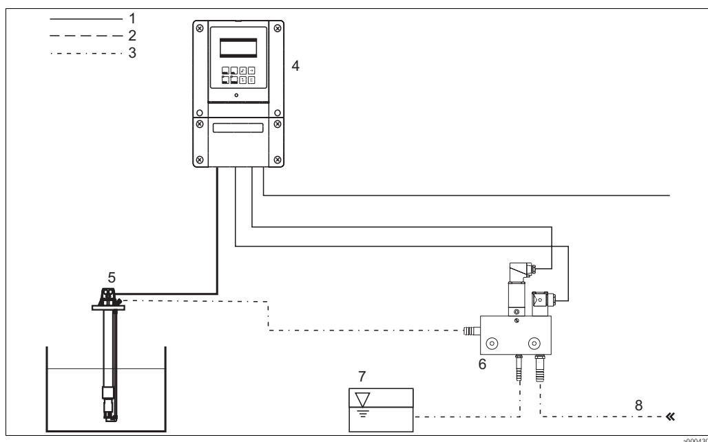
Fig. 57: Chemoclean cleaning
