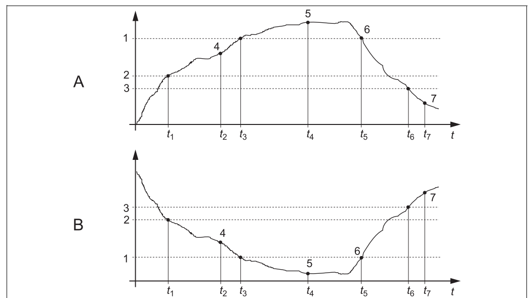
Fig. 55: Illustration of the alarm value and limit value functions
