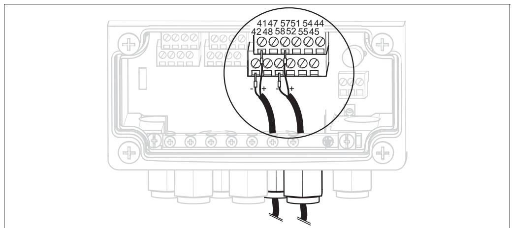
Fig. 35: Relay connection
