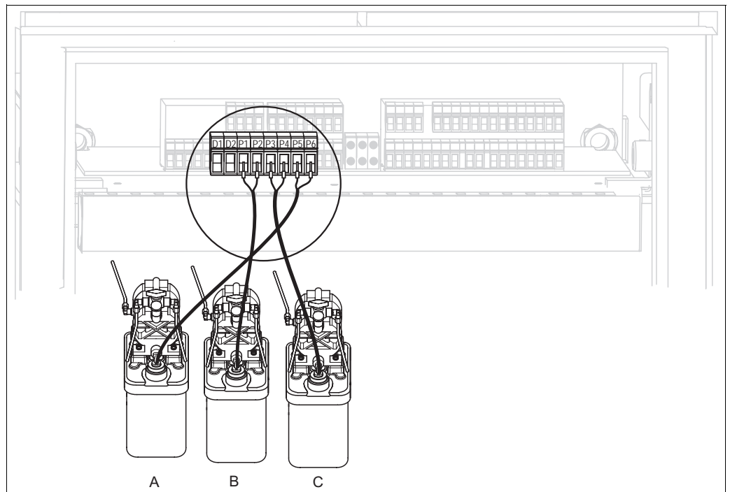
Fig. 20: Connecting level probes for buffer and cleaner
