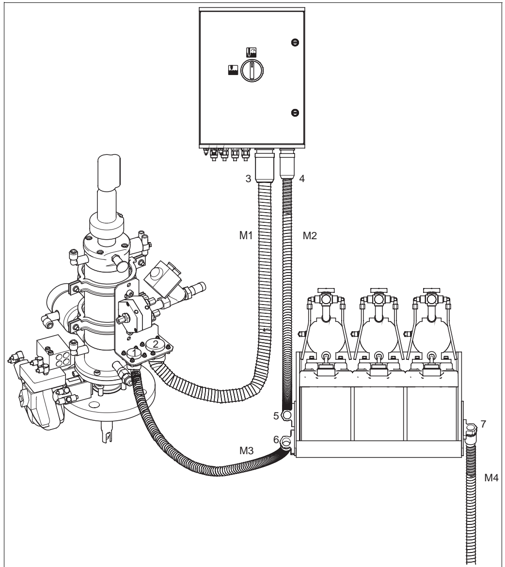
Fig. 42: Connecting multihoses
