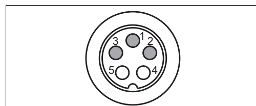
Fig. 74: Multihose socket M2 (Pg 21) at hose
