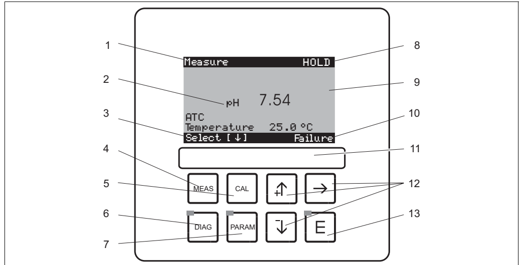
Fig. 51: Operating elements
