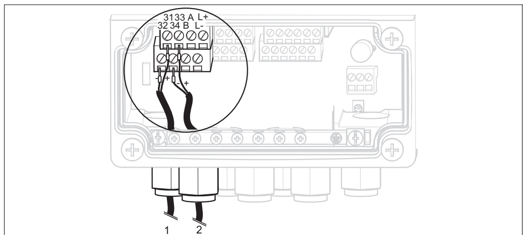
Fig. 32: Connecting current outputs
