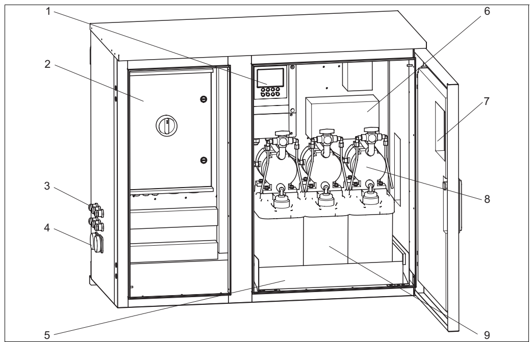
Fig. 62: Interior view of housing CYC310, stainless steel version
