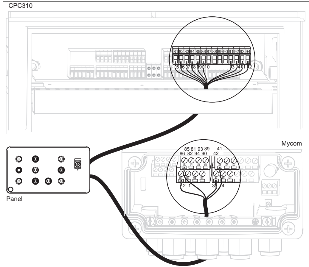
Fig. 66: Operating panel wiring
