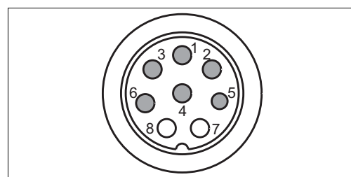
Fig. 72: Multihose socket M1 (Pg 29) at hose
