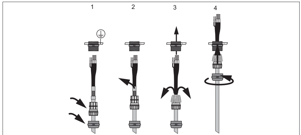
Fig. 30: Outer screen connection with metal cable gland
