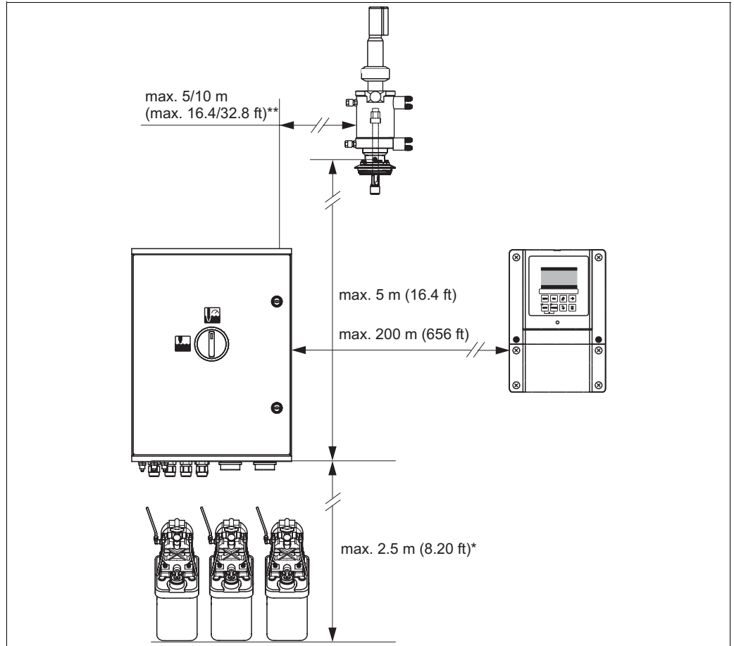
Fig. 3: Maximum spacing for Topcal S CPC310 system components
