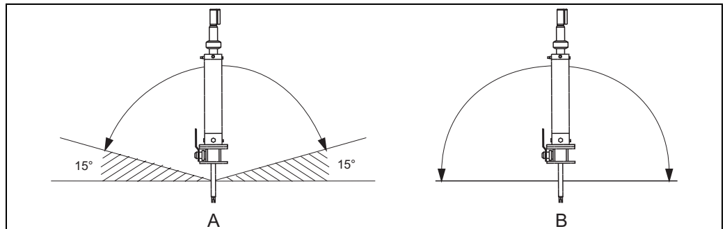
Fig. 4: Permitted orientation depending on the sensor used
