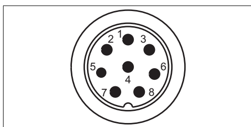
Fig. 71: Multihose connector M1 (Pg 29) at housing
