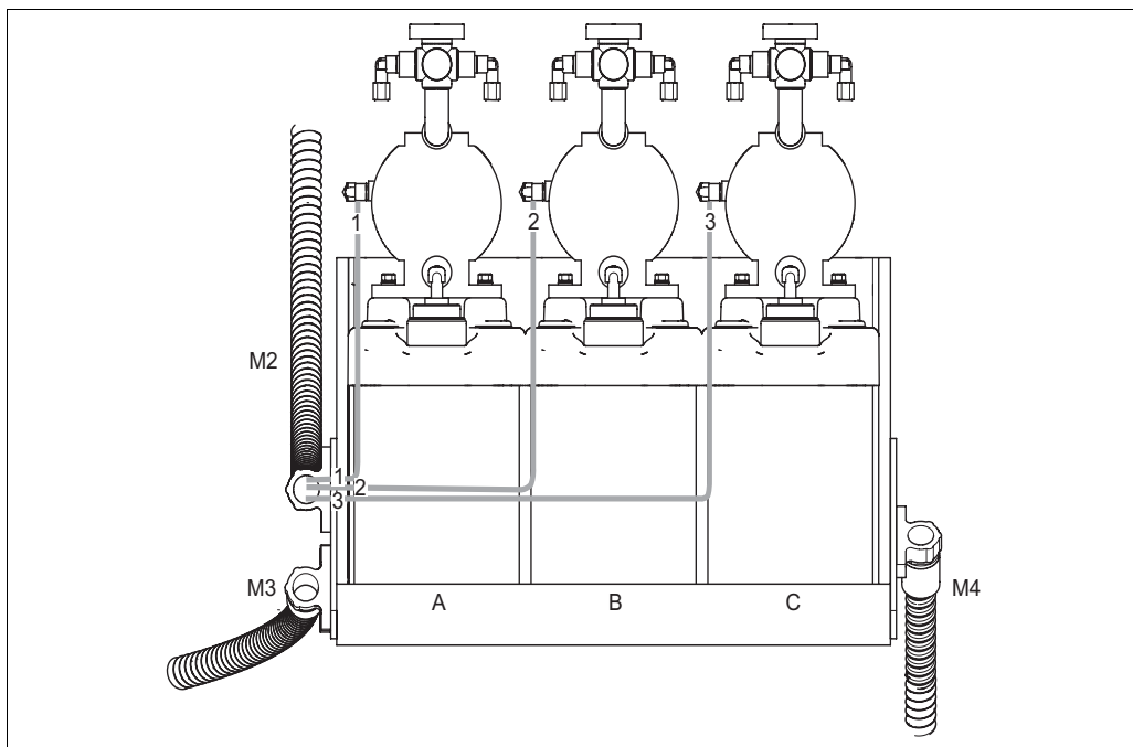
Fig. 48: Compressed air control of the membrane pumps
