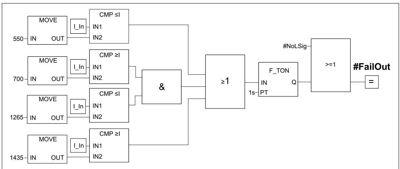
25 Function block, error current analysis
