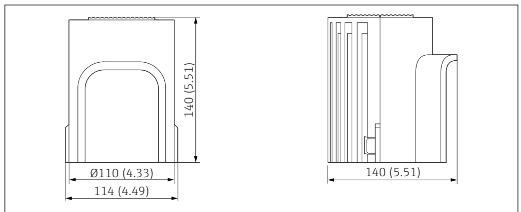
46 Dimensions of weather protection cover PBT. Unit of measurement mm (in)
