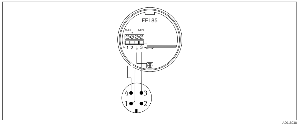
19 Terminal assignment with M12 connector, minimum detection mode of operation
