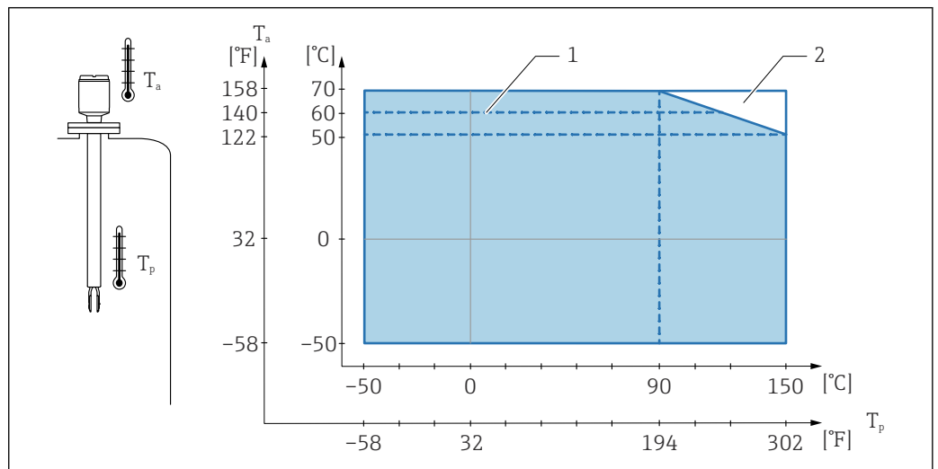
47 Permitted ambient temperature T_a at the housing as a function of the process temperature T_p in the vessel; maximum process temperature 150 °C ( 302 °F)
