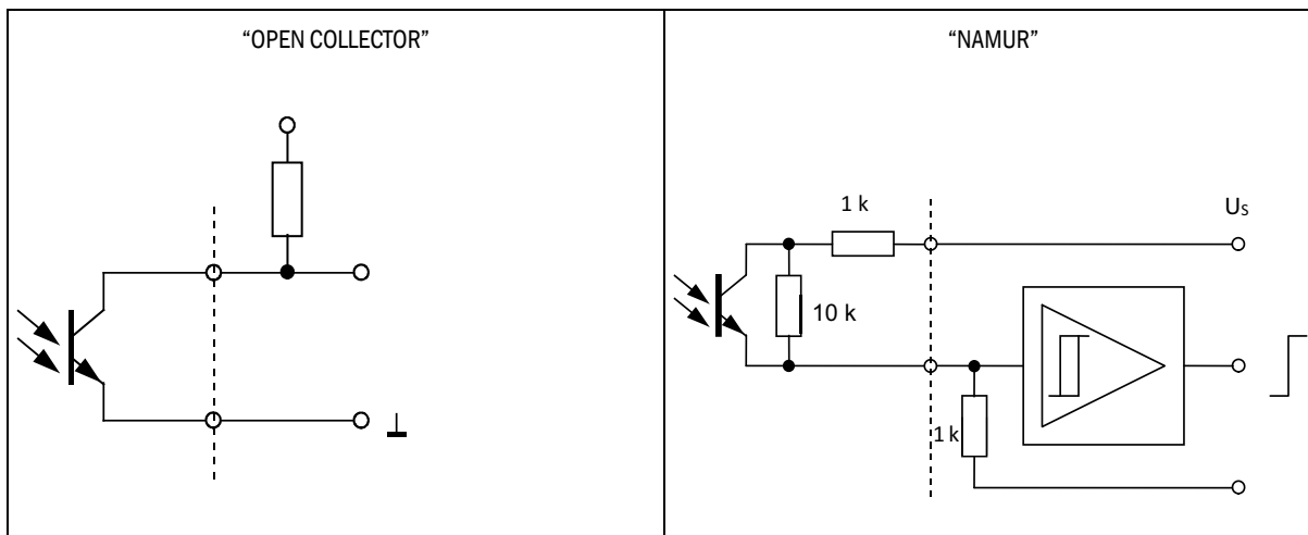
Figura 90 Circuito DO (Open Collector - Namur)
