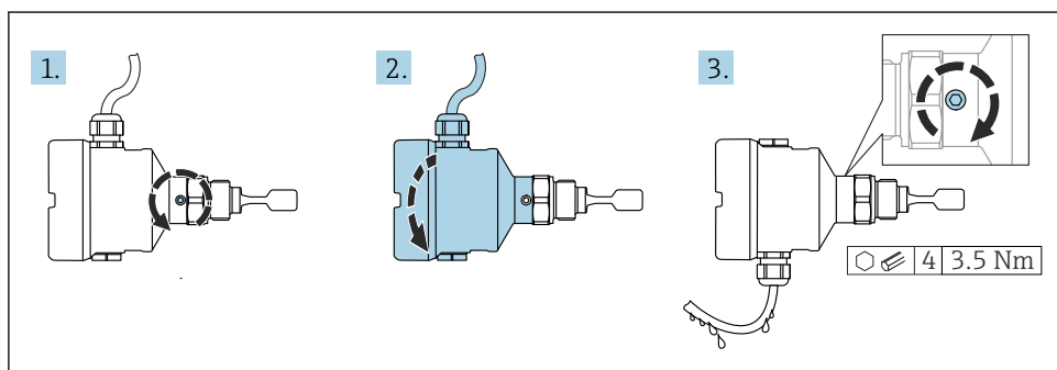
17 Housing with external locking screw and drip loop
