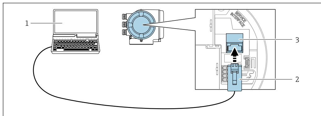
36 Raccordement via interface service (CDI-RJ45)
