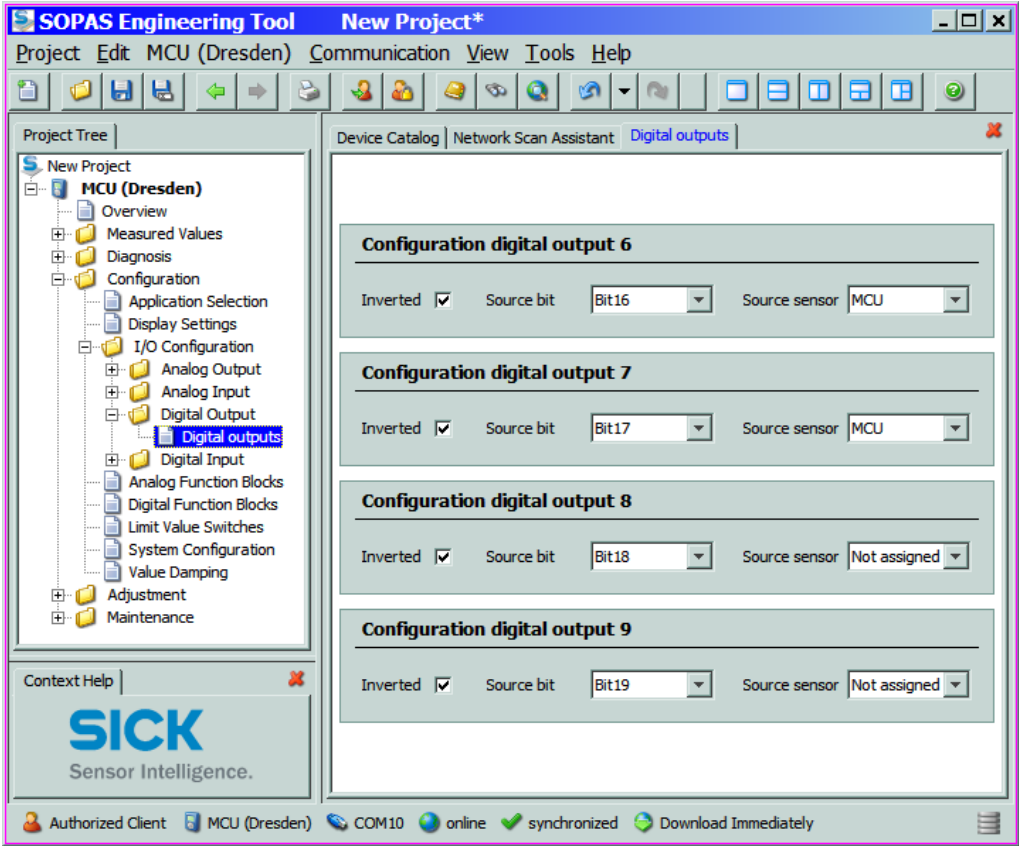
Figura 71 Direttorio "Configuration / I/O Configuration / Digital Output / Digital outputs"
