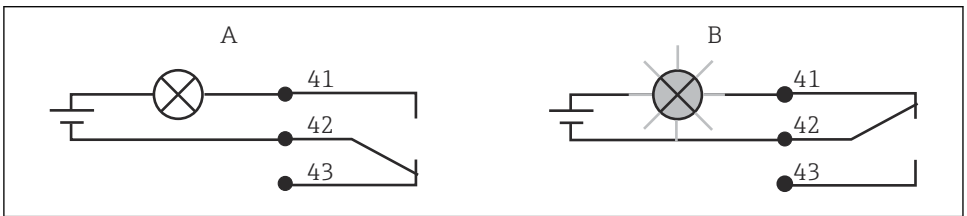
12 Recommended fail-safe switching for the alarm contact
