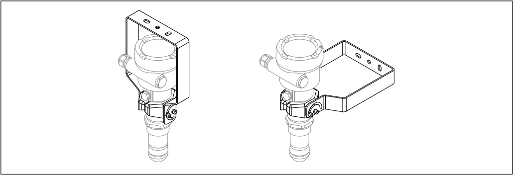
41 Mounting bracket adjustable FMR6xB; ceiling or wall mounting
