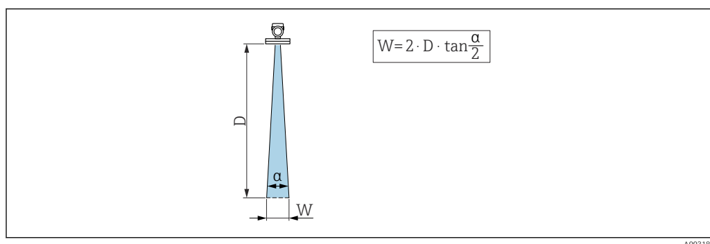
8 Relationship between beam angle \alpha , distance D and beamwidth diameter W
