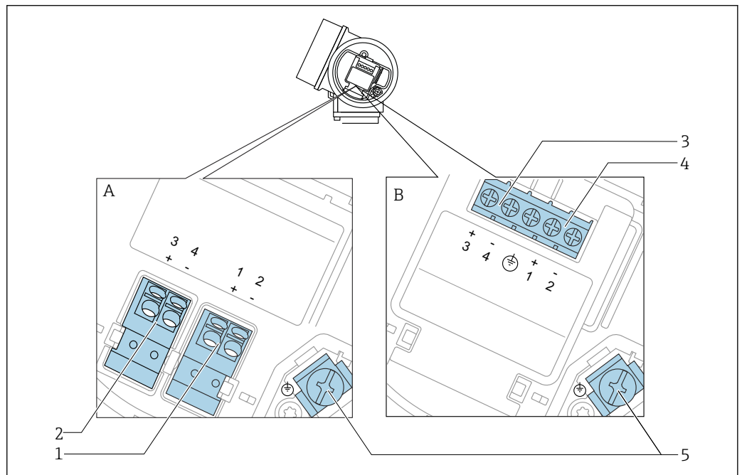
12 接线端子分配: PROFIBUS PA / FOUNDATION Fieldbus
