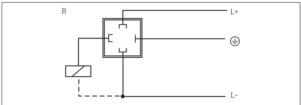
6 Device with M16x1.5 valve connector or NPT 1/2"
