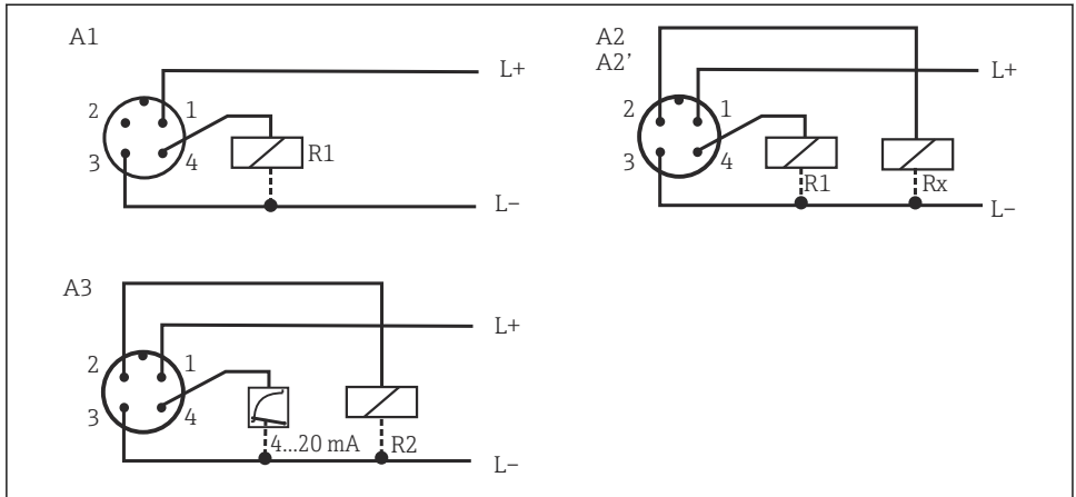
5 Device with M12x1 connector
