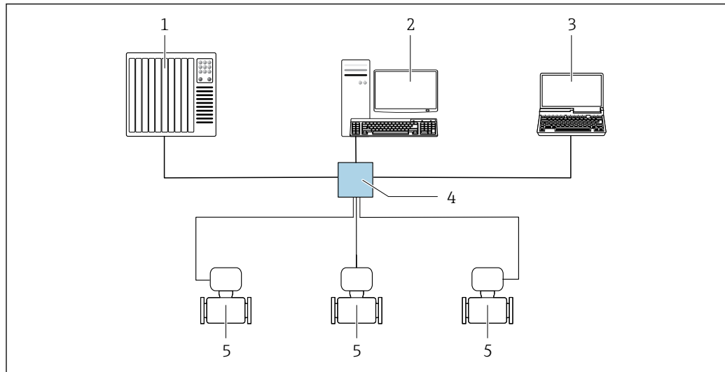
50 Options for remote operation via Ethernet/IP network: star topology
