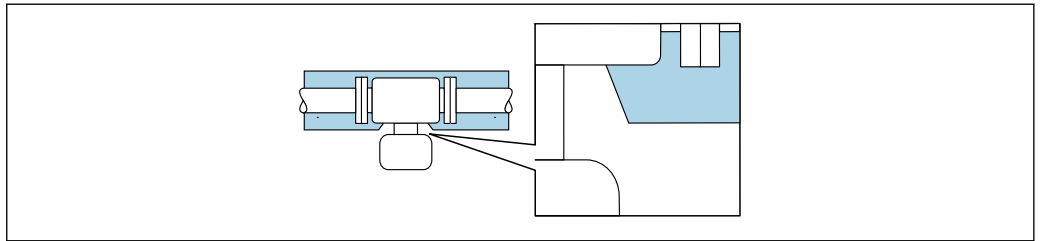
26 Thermal insulation with exposed extended neck
