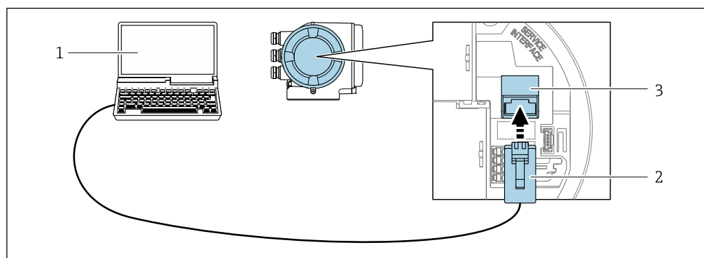
54 Connection via service interface (CDI-RJ45)
