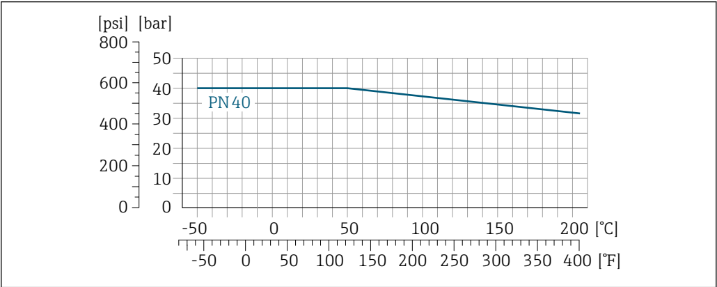
17 With flange material 1.4404 (F316/F316L)
