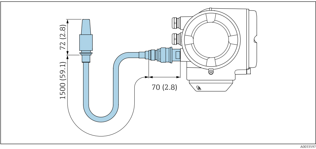
38 Unit mm (in)
