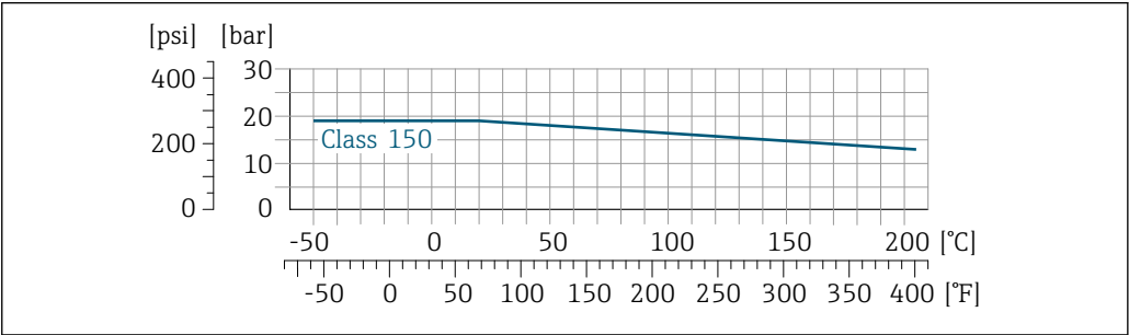
18 With flange material 1.4404 (F316/F316L)
