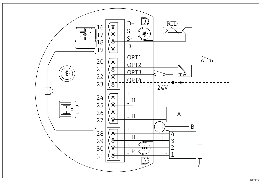
9 NRF590 (intrinsically safe) terminals
