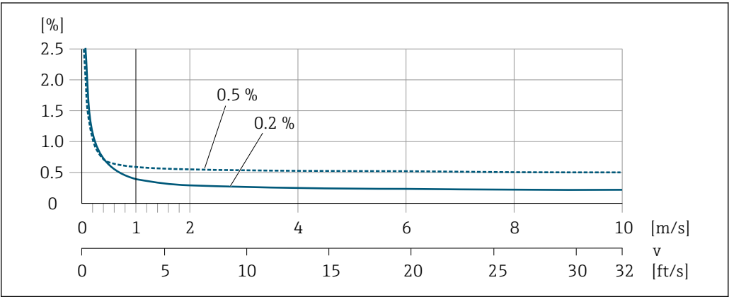
13 Maximum measurement error in % o.r.
