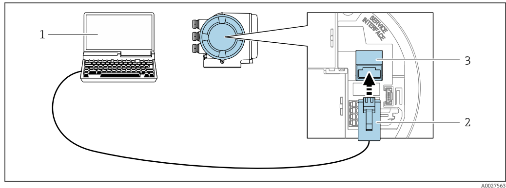
75 Connection via service interface (CDI-RJ45)
