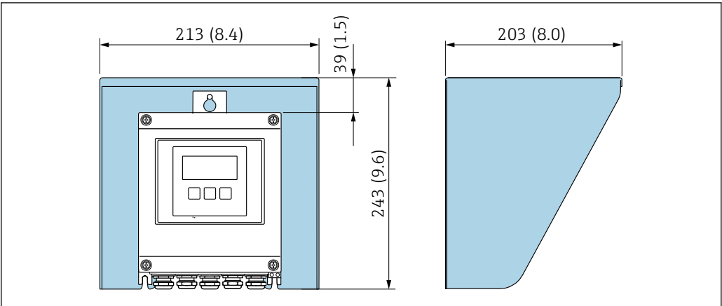
21 Protective cover for Proline 500 – digital; unit mm (in)
