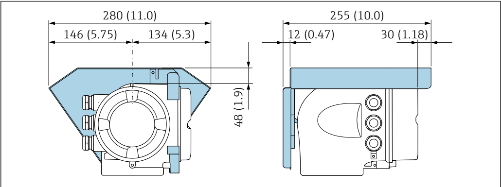
54 Protective cover for Proline 500; unit mm (in)
