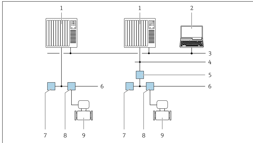
64 Options for remote operation via FOUNDATION Fieldbus network
