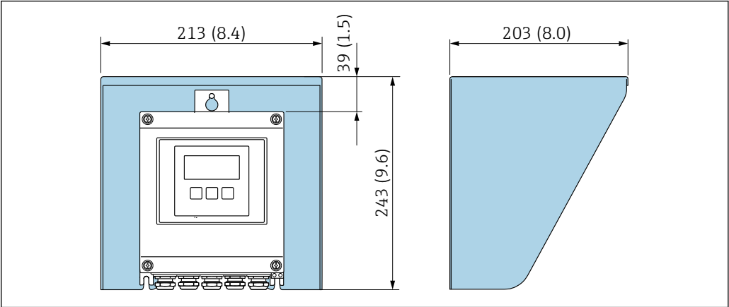
53 Protective cover for Proline 500 – digital; unit mm (in)
