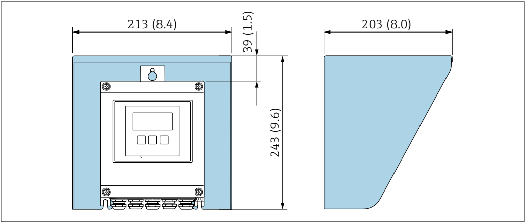
45 Protective cover for Proline 500 – digital; unit mm (in)
