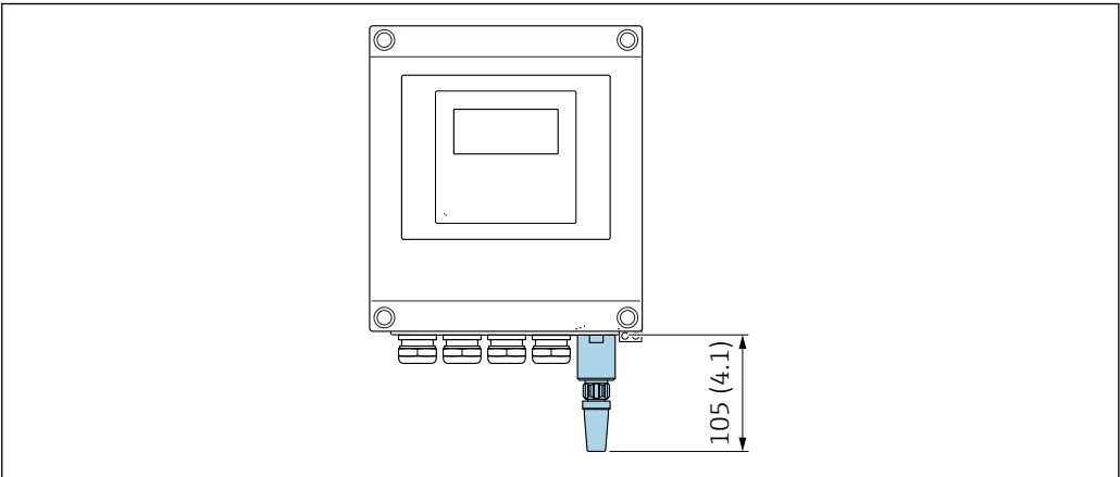
55 Unit mm (in)
