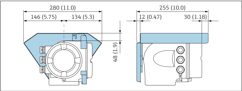
22 Protective cover for Proline 500; unit mm (in)
