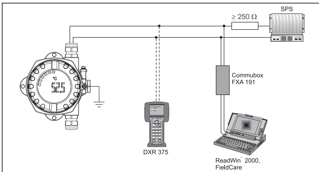
Fig. 7: HART® connection using other power supplies
