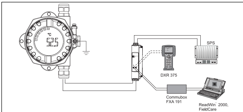
Fig. 6: HART® connection with the E+H power supply RN 221N
