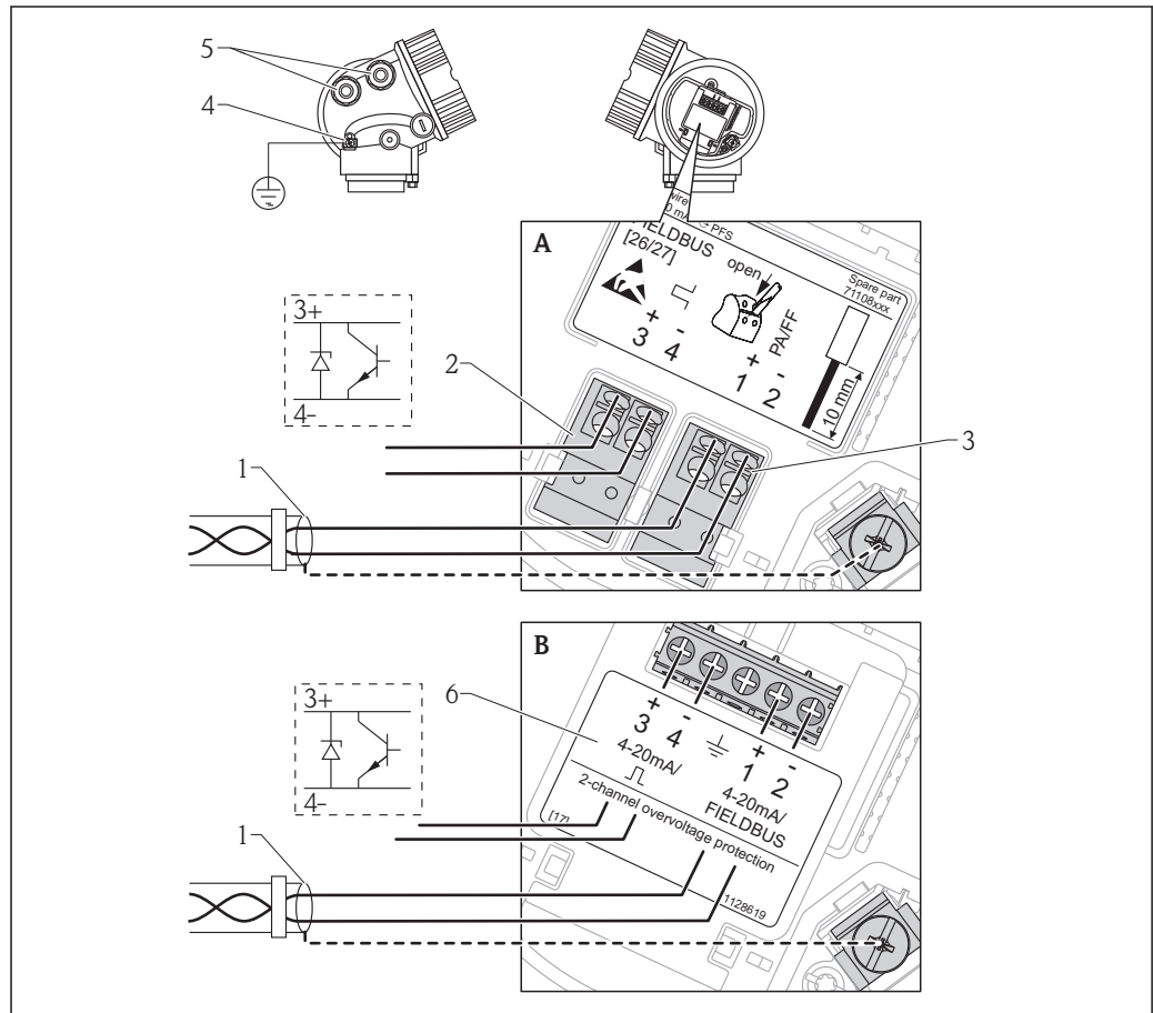
9 Occupation des bornes PROFIBUS PA / FOUNDATION Fieldbus
