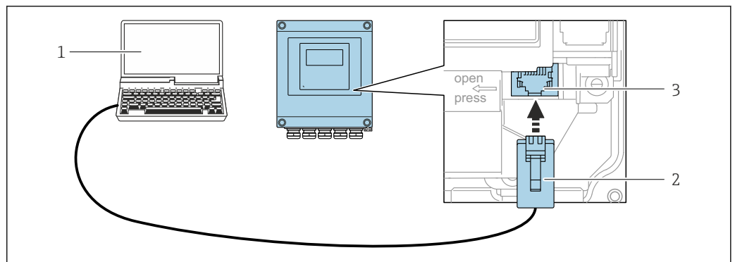
62 Raccordement via interface service (CDI-RJ45)
