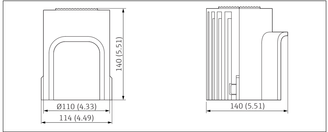
38 Dimensions of weather protection cover PBT. Unit of measurement mm (in)
