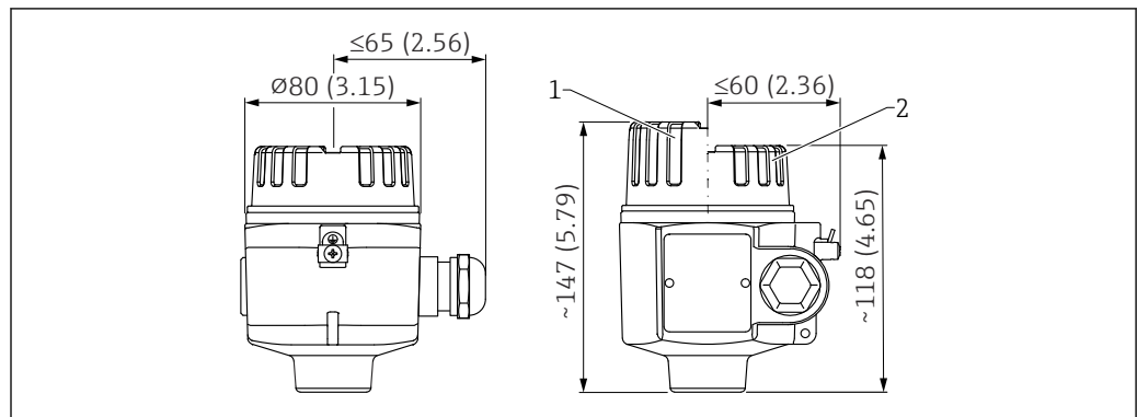
31 Dimensions of 316L housing, with adapter screwed onto sensor. Unit of measurement mm (in)
