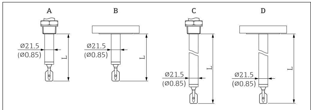
33 Sensor length L. Unit of measurement mm (in)
