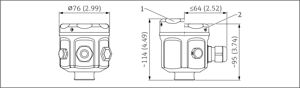
28 Dimensions of 316L housing, hygienic. Unit of measurement mm (in)
