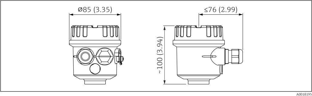
27 Dimensions of plastic housing. Unit of measurement mm (in)
