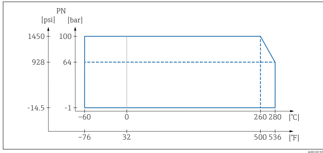
25 Process pressure range for high-temperature version with 230 °C (450 °F)/280 °C (540 °F)
