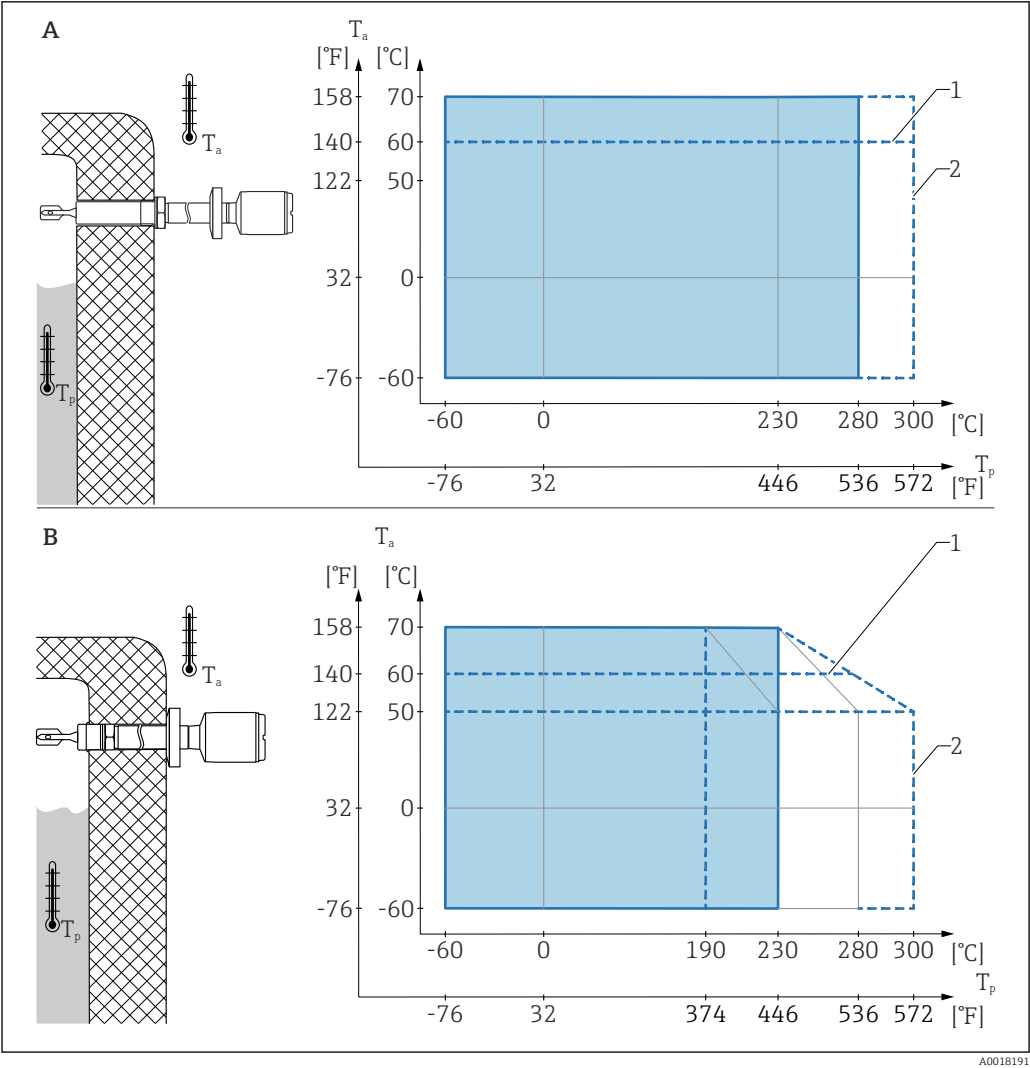
23 Permitted ambient temperature T_a at the housing as a function of the process temperature T_p in the vessel; maximum process temperature 230 °C (446 °F) or 280 °C (536 °F)
