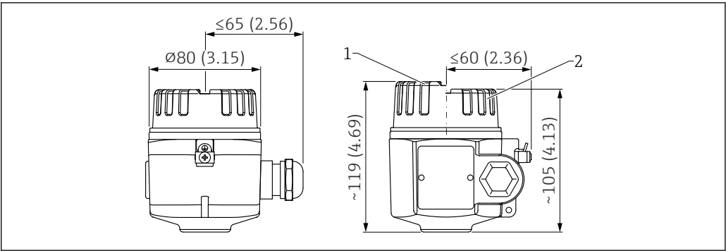
29 Dimensions of aluminum housing. Unit of measurement mm (in)
