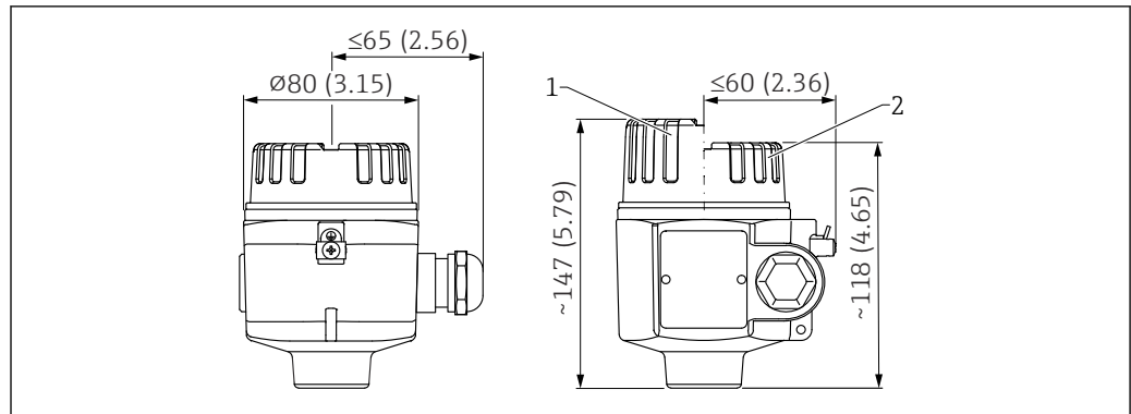
30 Dimensions of aluminum housing, with adapter screwed onto sensor. Unit of measurement mm (in)
