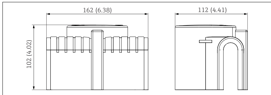
37 Dimensions of weather protection cover PA6. Unit of measurement mm (in)
