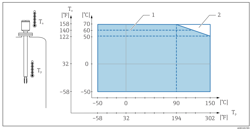
22 Permitted ambient temperature T_a at the housing as a function of the process temperature T_p in the vessel; maximum process temperature 150 °C (302 °F)
