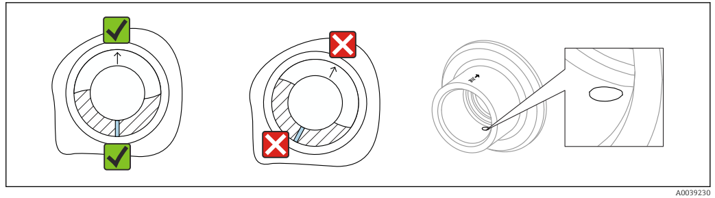
21 Weld-in adapter with leakage hole
