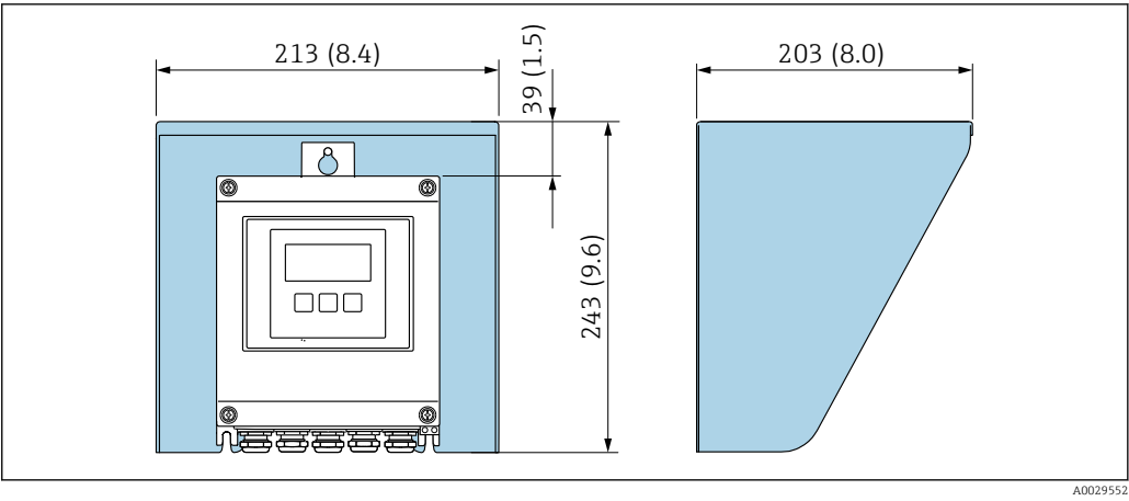
19 Protective cover for Proline 500 – digital; unit mm (in)
