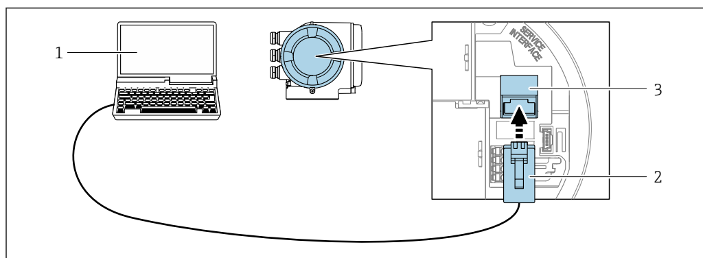
52 Raccordement via interface service (CDI-RJ45)
