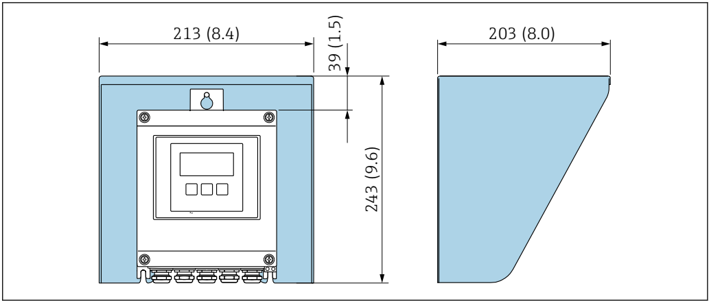
36 Weather protection cover for Proline 500 – digital; unit mm (in)
