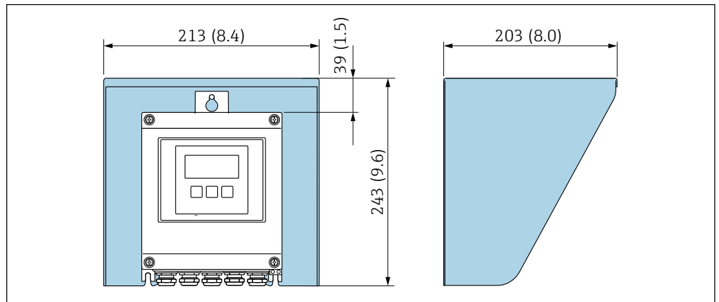
42 Weather protection cover for Proline 500 – digital; unit mm (in)
