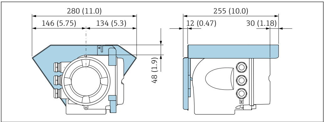
37 Weather protection cover for Proline 500 – unit mm (in)
