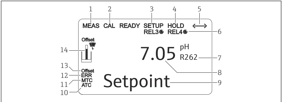
9 Transmitter LC-display
