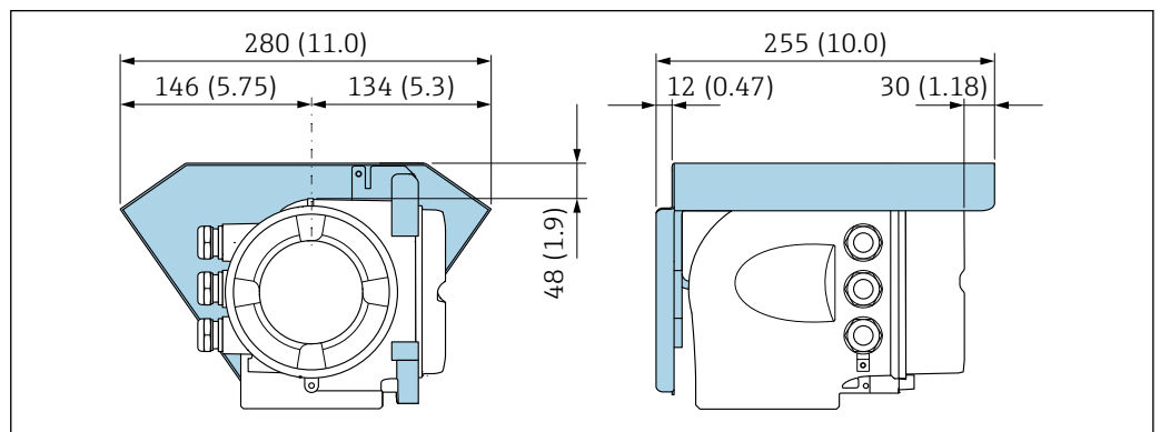
20 Protective cover for Proline 500; unit mm (in)
