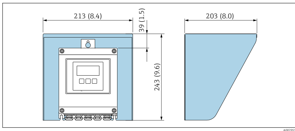
26 Protective cover for Proline 500 – digital; unit mm (in)
