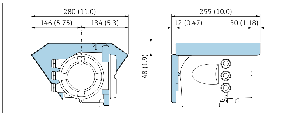
27 Protective cover for Proline 500; unit mm (in)
