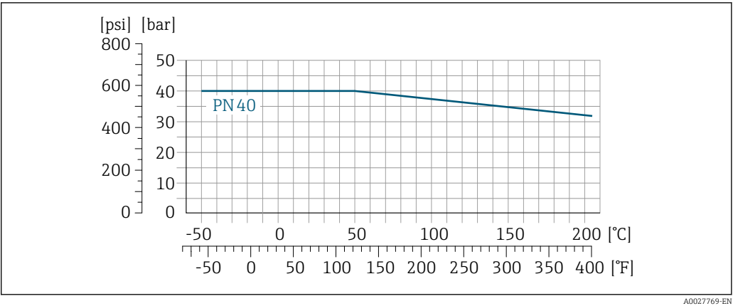
22 With flange material 1.4301 (304); wetted parts: zirconium 702, tantalum
