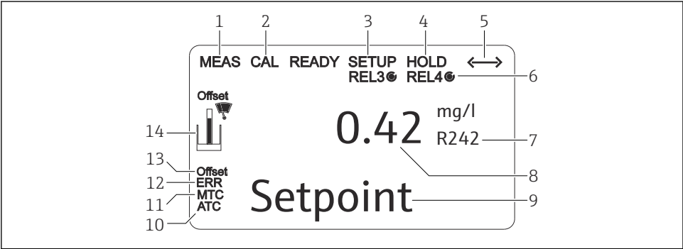
15 Transmitter LC-display
