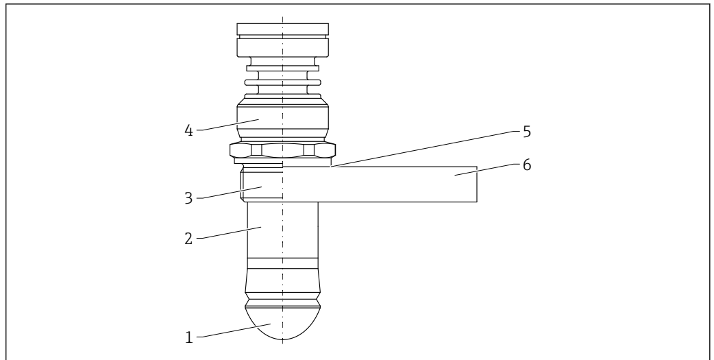
59 Material; Drip-off Antenne 50 mm (2 in)
