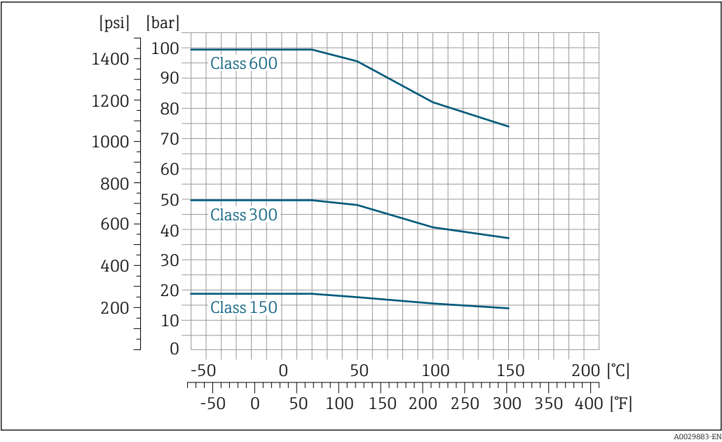
22 With flange material 1.4301 (304); wetted parts: titanium
