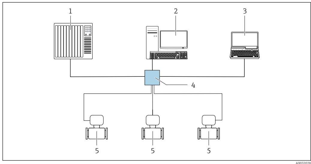
56 Options for remote operation via Modbus TCP over Ethernet - 100 Mbit/s: Star topology
