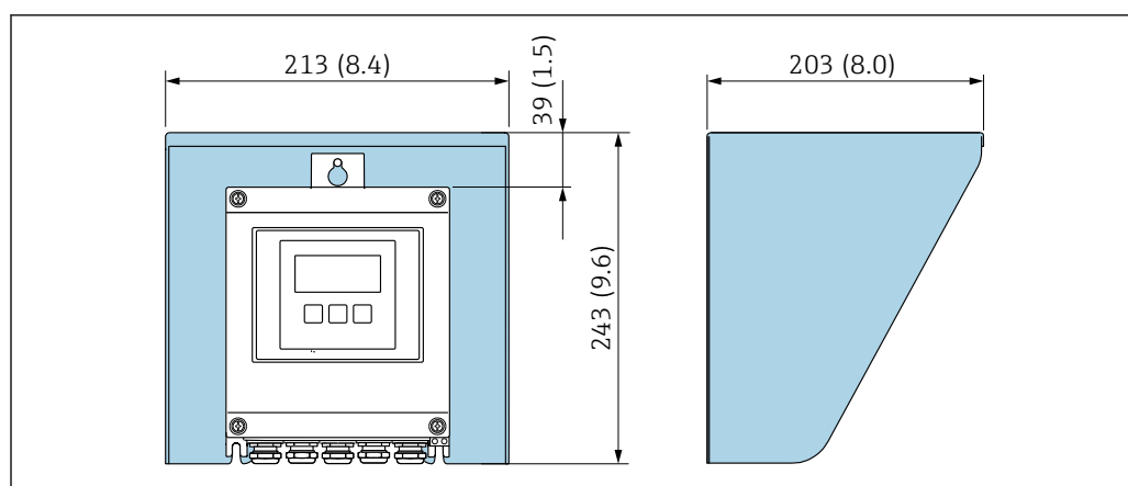
37 Weather protection cover for Proline 500 – digital; unit mm (in)
