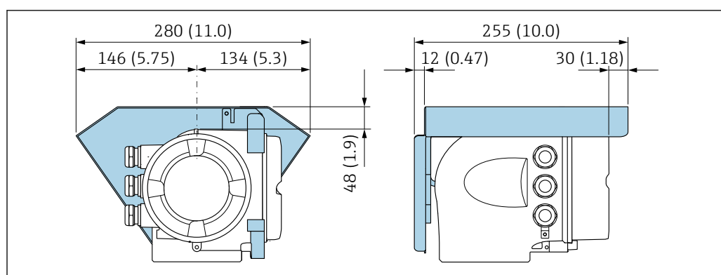
38 Weather protection cover for Proline 500 – unit mm (in)
