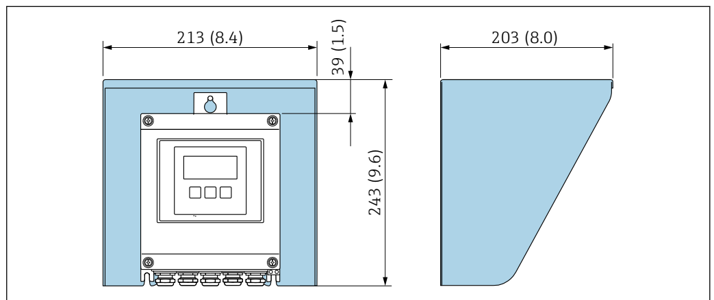
18 Weather protection cover for Proline 500 – digital; unit mm (in)
