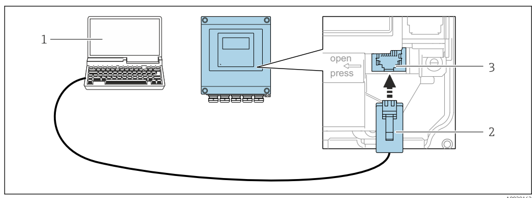
57 Connection via service interface (CDI-RJ45)
