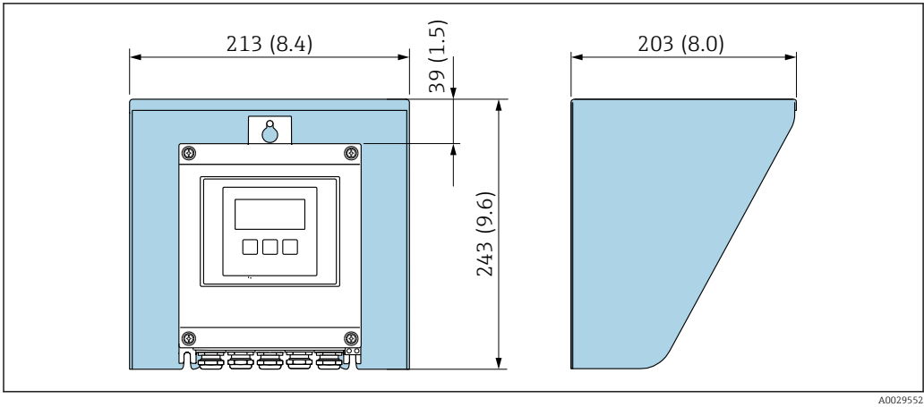
31 Weather protection cover for Proline 500 – digital; unit mm (in)
