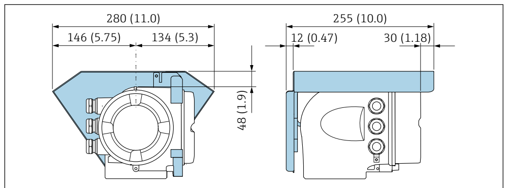
19 Weather protection cover for Proline 500 – unit mm (in)
