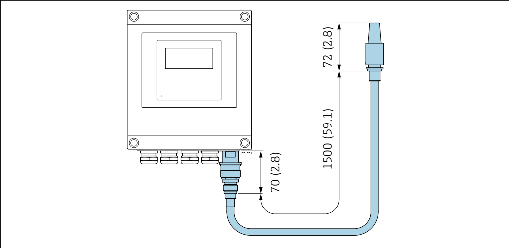
34 Unit mm (in)
