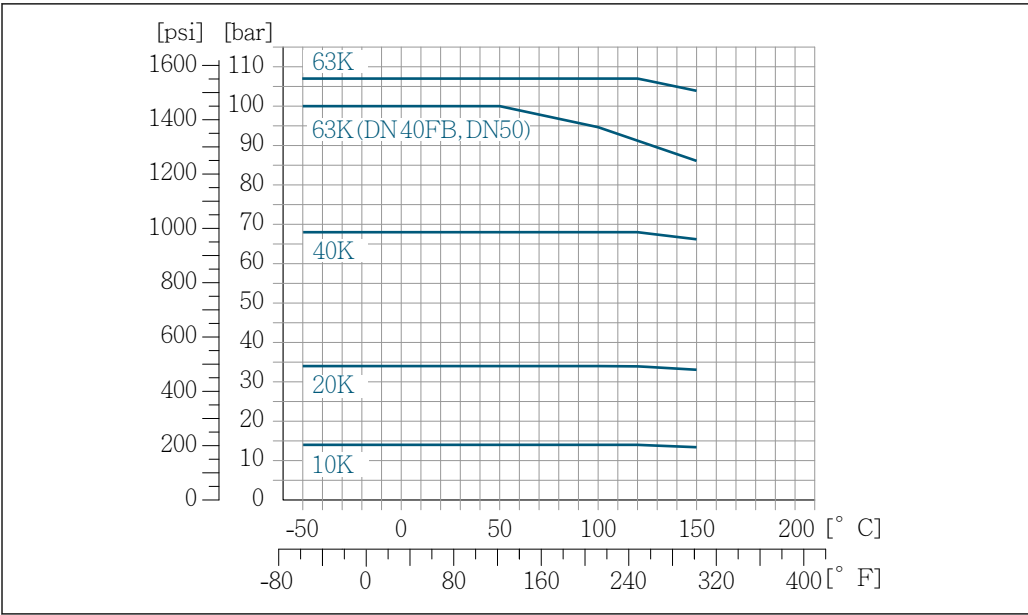
23 With flange material 1.4301 (304). Wetted parts: titanium.
