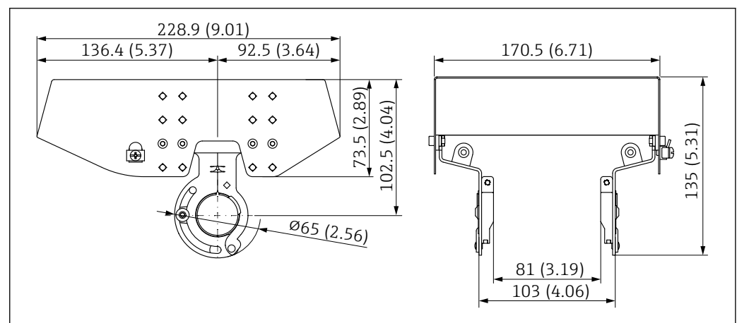
64 Dimensions of weather protection cover, 316 L, XW112. Unit of measurement mm (in)
